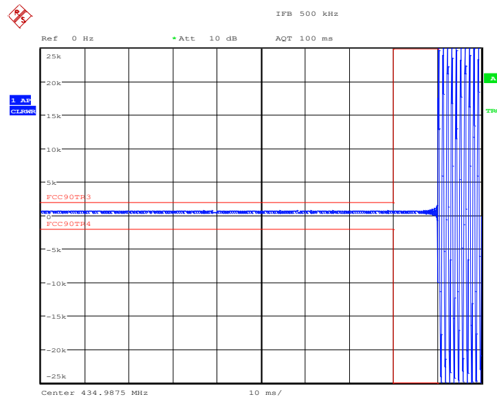
Figure 30- Switch On Transient, 434.9875 MHz
