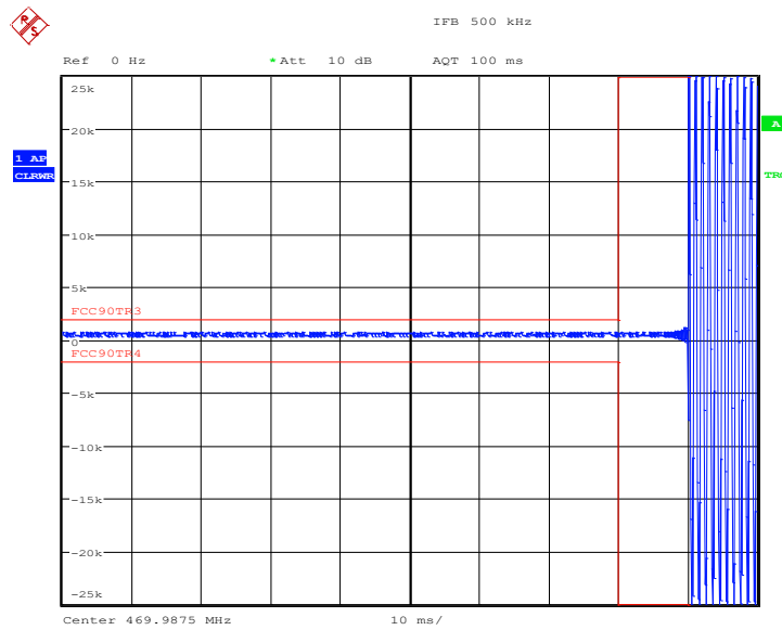
Figure 32 - Switch On Transient, 469.9875 MHz
