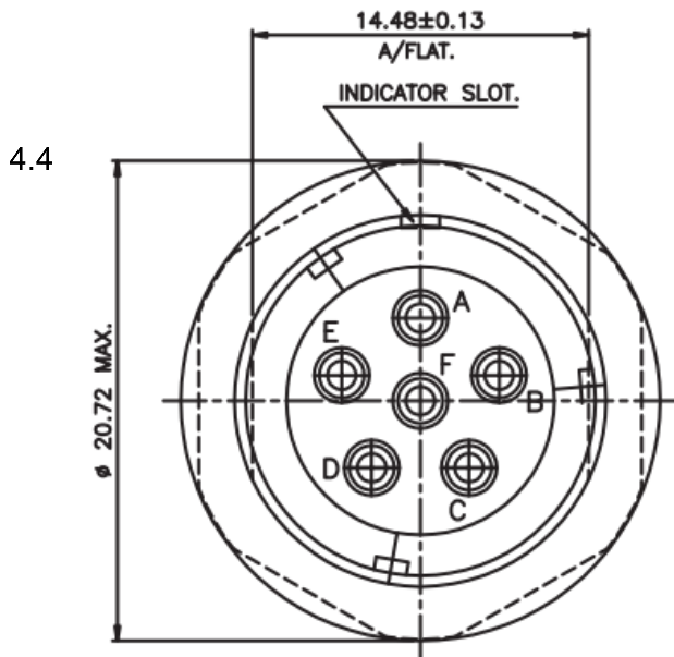
Figure 4-1 Amphenol 164 series 6 pin connector variant
