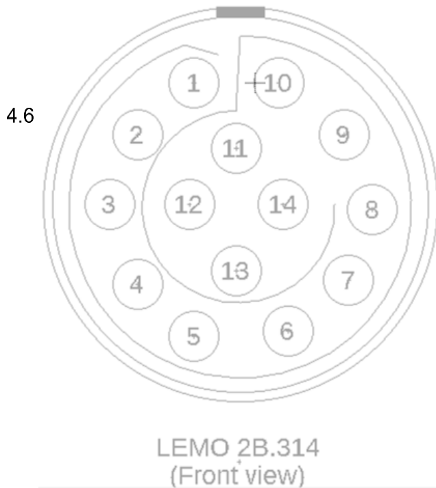
Figure 4-3 Lemo 14 pin connector variant
