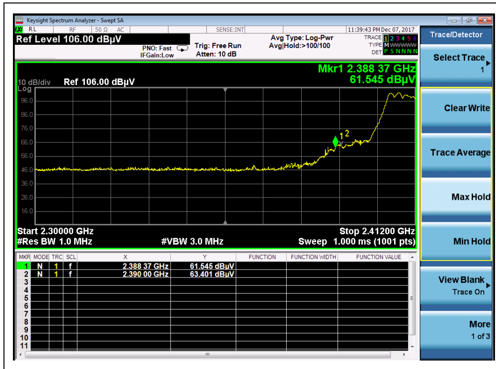
(Channel = 3 PEAK @ 802.11n-40)
