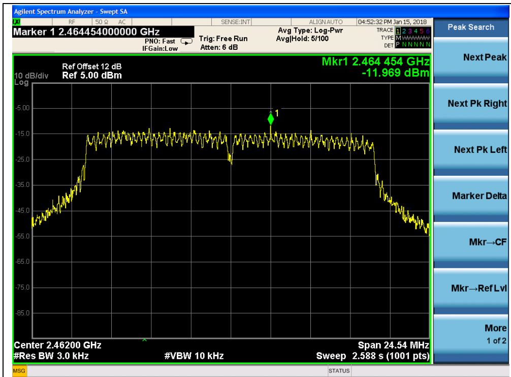
(Channel = 11 @ 802.11n-20MHz, ANT0)
