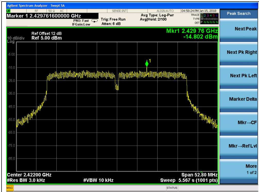
(Channel = 3 @ 802.11n-40MHz, ANT1)
