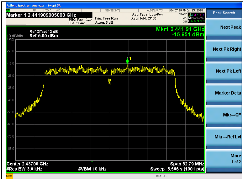
(Channel = 6 @ 802.11n-40MHz, ANT1)
