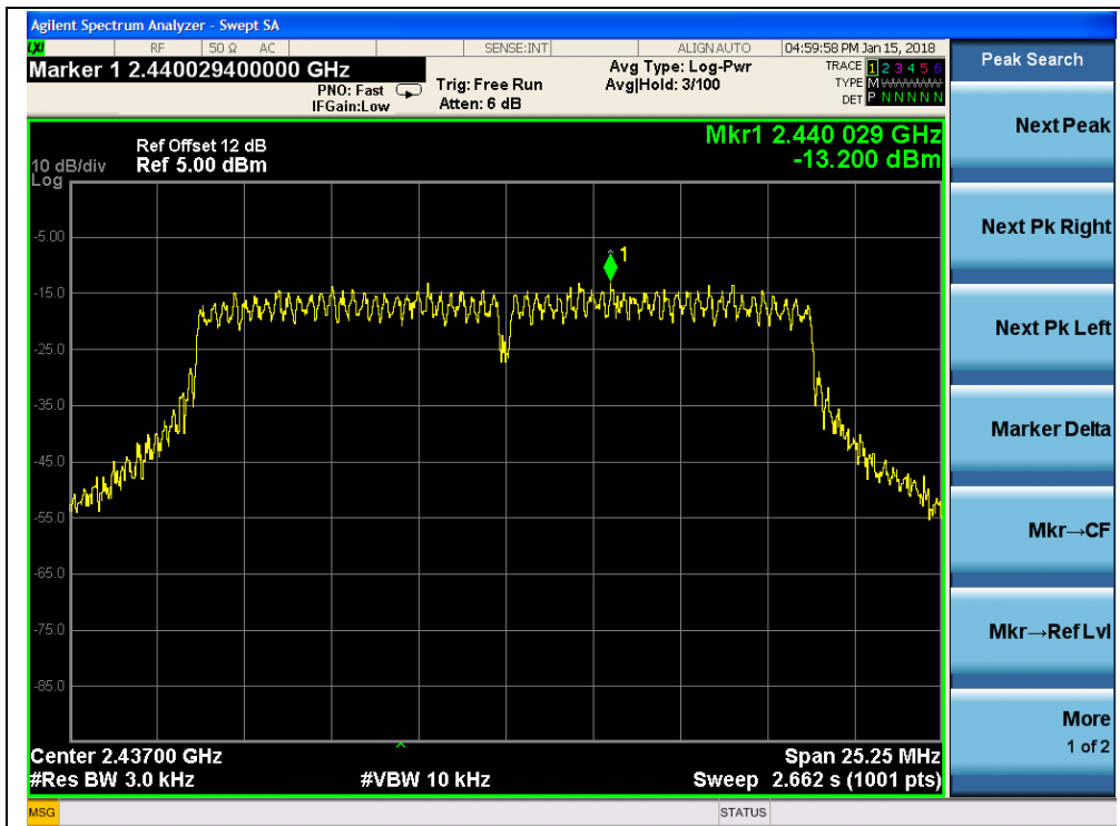
(Channel = 6 @ 802.11n-20MHz, ANT1)
