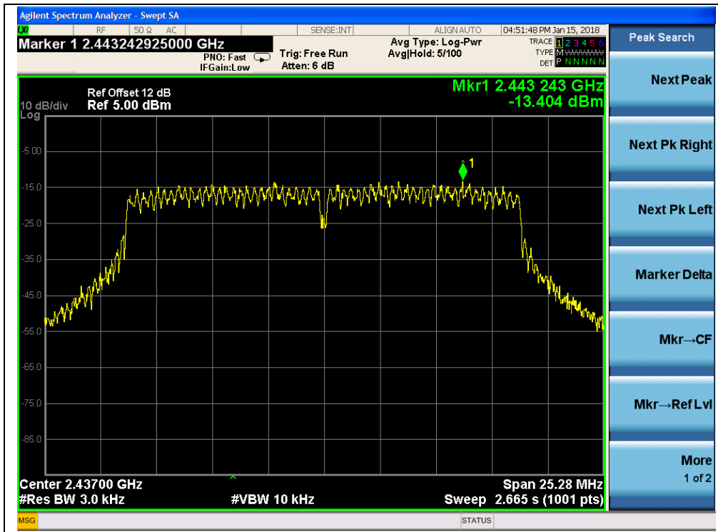
(Channel = 6 @ 802.11n-20MHz, ANT0)
