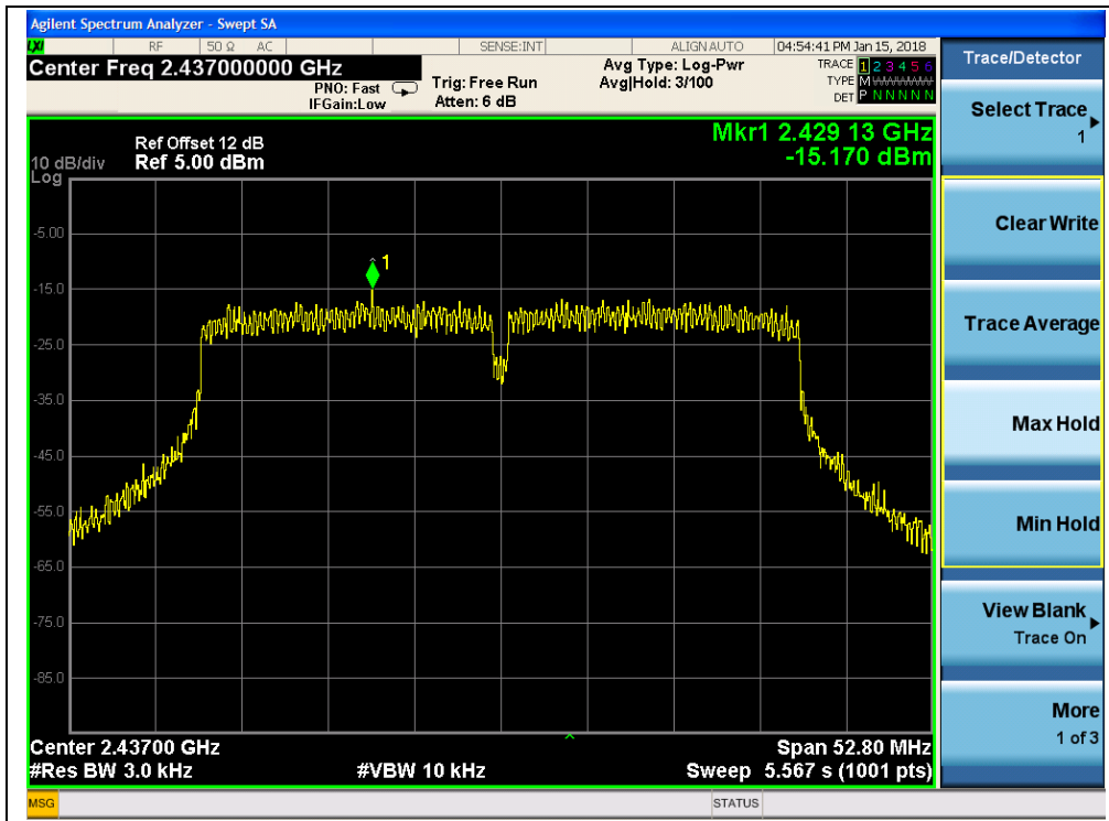
(Channel = 6 @ 802.11n-40MHz, ANT0)
