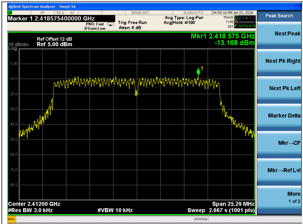
(Channel = 1 @ 802.11n-20MHz, ANT1)
