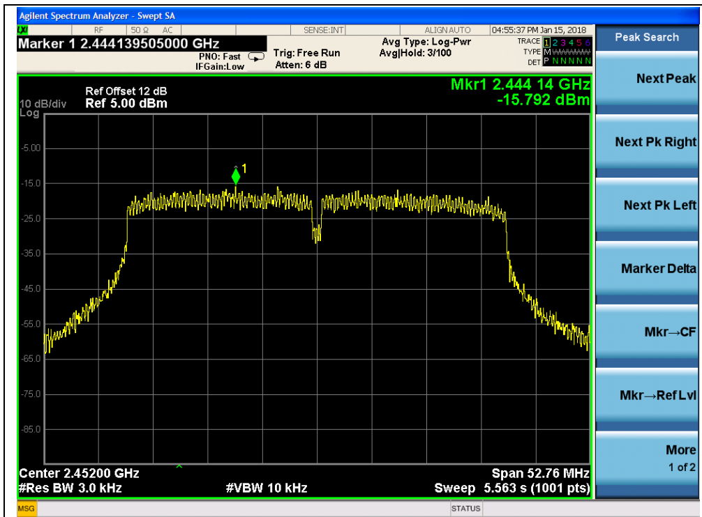
(Channel = 9 @ 802.11n-40MHz, ANT0)
