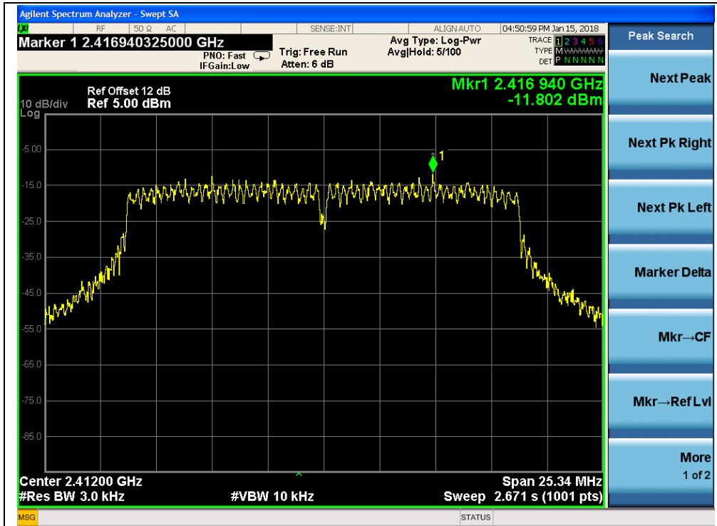
(Channel = 1 @ 802.11n-20MHz, ANT0)
