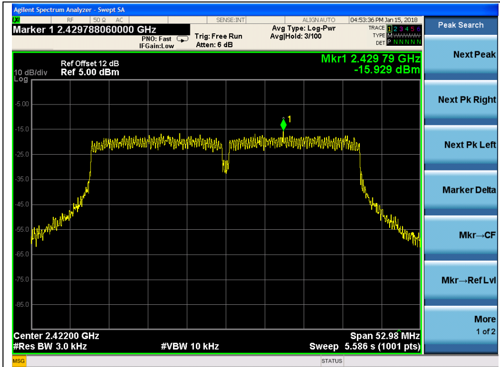
(Channel = 3 @ 802.11n-40MHz, ANT0)
