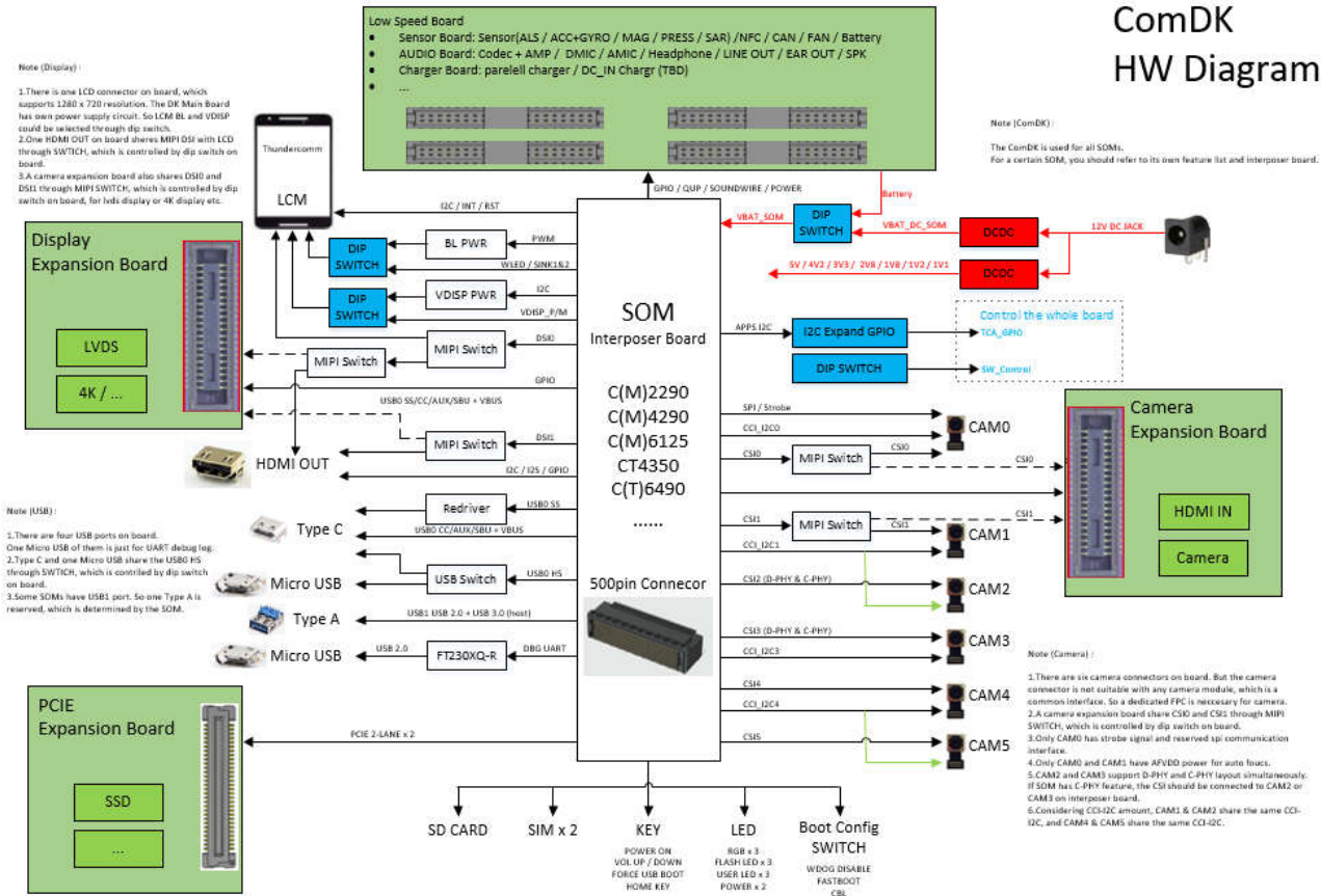
Figure 1-2. Main Board Block Diagram
