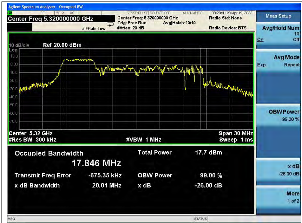
(Channel 64, 5320MHz, 802.11ax (HEW20) RU52)
