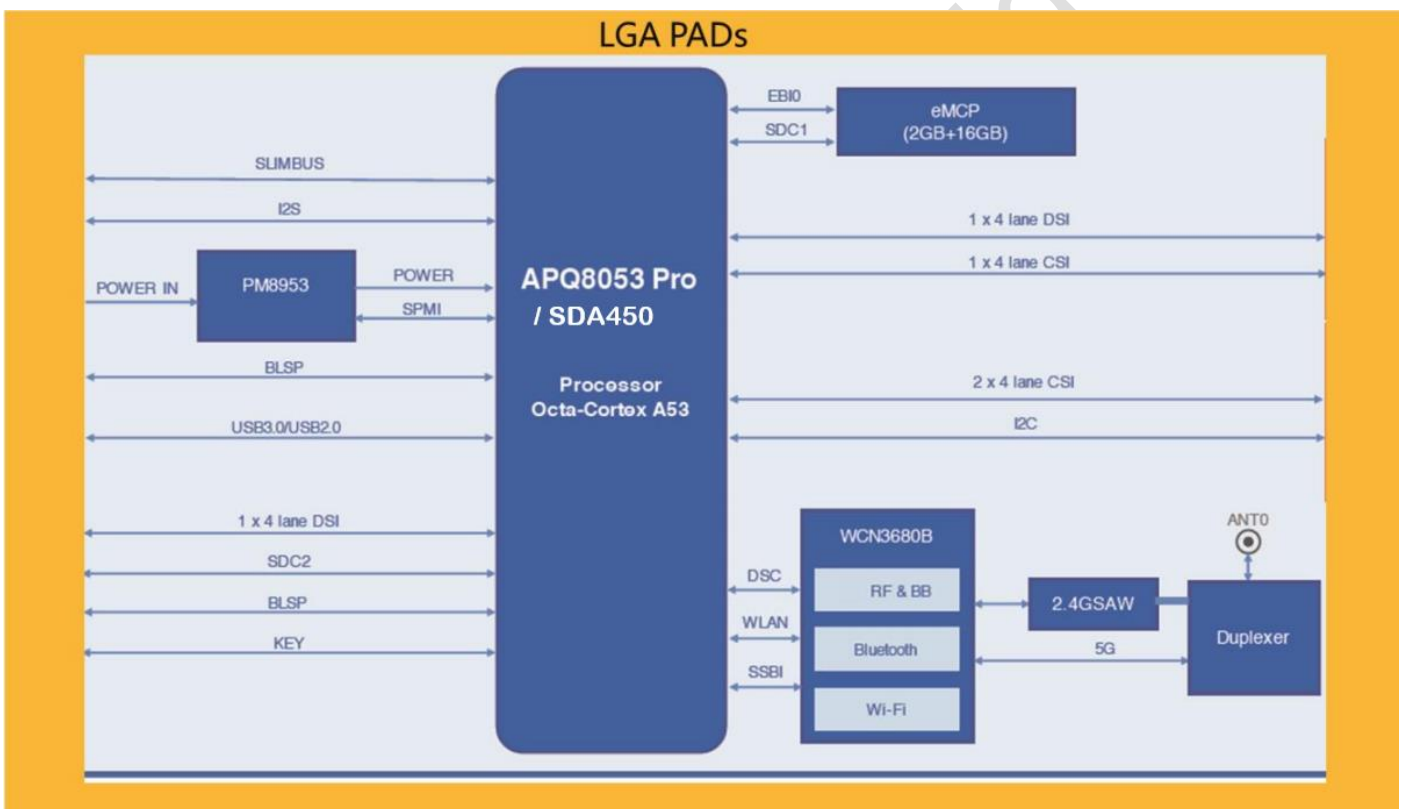
Figure 1-1. Block Diagram
