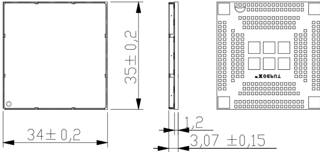
Figure 1-2. Chipset Overview
