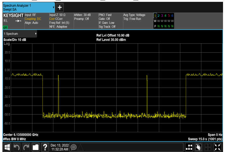
6.4G_ax20_6135MHz_Chain1_Interferer1dBloweroccur
