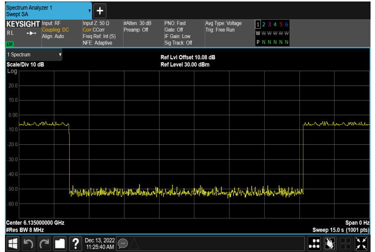
6.4G_ax20_6135MHz_Chain1_Interferer1dBloweroccur
