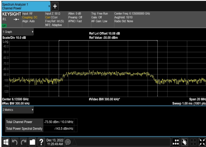
6.4G_ax20_6135MHz_Chain1_ThresholdLevel
