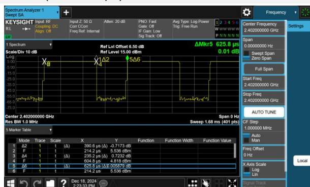
GFSK (BLE 1Mbps)
