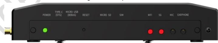
Figure 2-2. Front View
