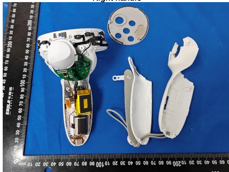
Right handle
