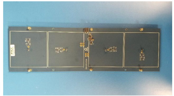
830-00012_REV1_RBK60xx_sub6SURF_CIRCUITS_TOP
