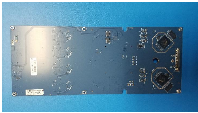
830-00010_REV4_RBK6028_mmwSURF_BOT
