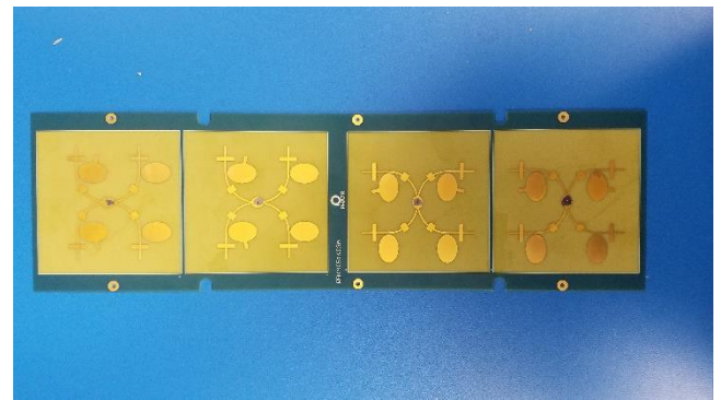
170-00014_REV1_RBK60xx_sub6SURF_ANTENNA_TOP
