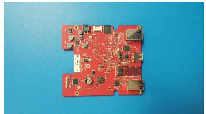
830-00011_REV3_RBK60xx_PROCESSOR_TOP
