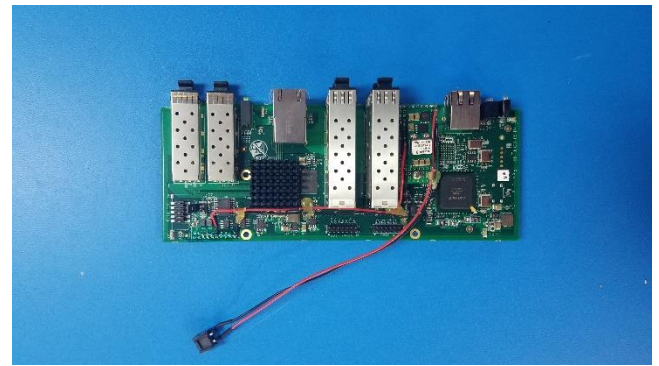
820-00028_REV1_RBK60xx_SWITCH_TOP
