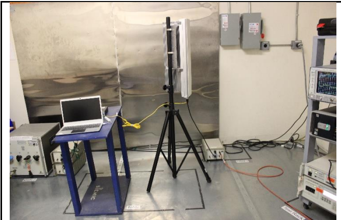
Conducted Emissions – Front View
