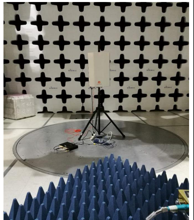
Radiated Emissions (>1GHz) – Rear View
