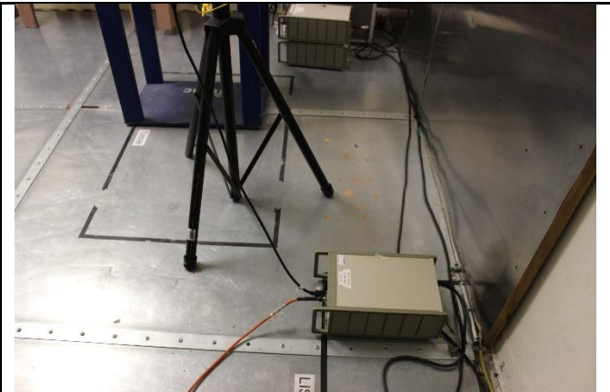
Conducted Emissions – Rear View
