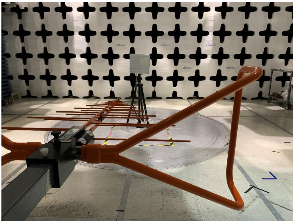
Radiated Emissions below 1GHz Front View
