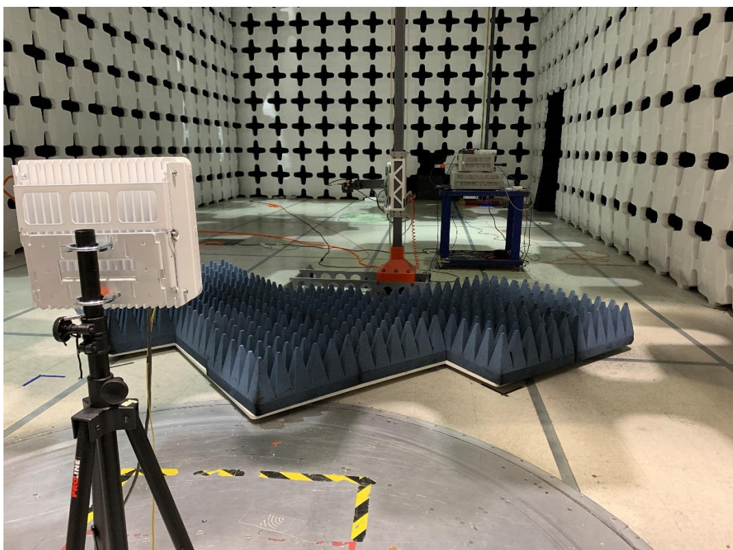
Radiated Emissions 18-40GHz Front View
