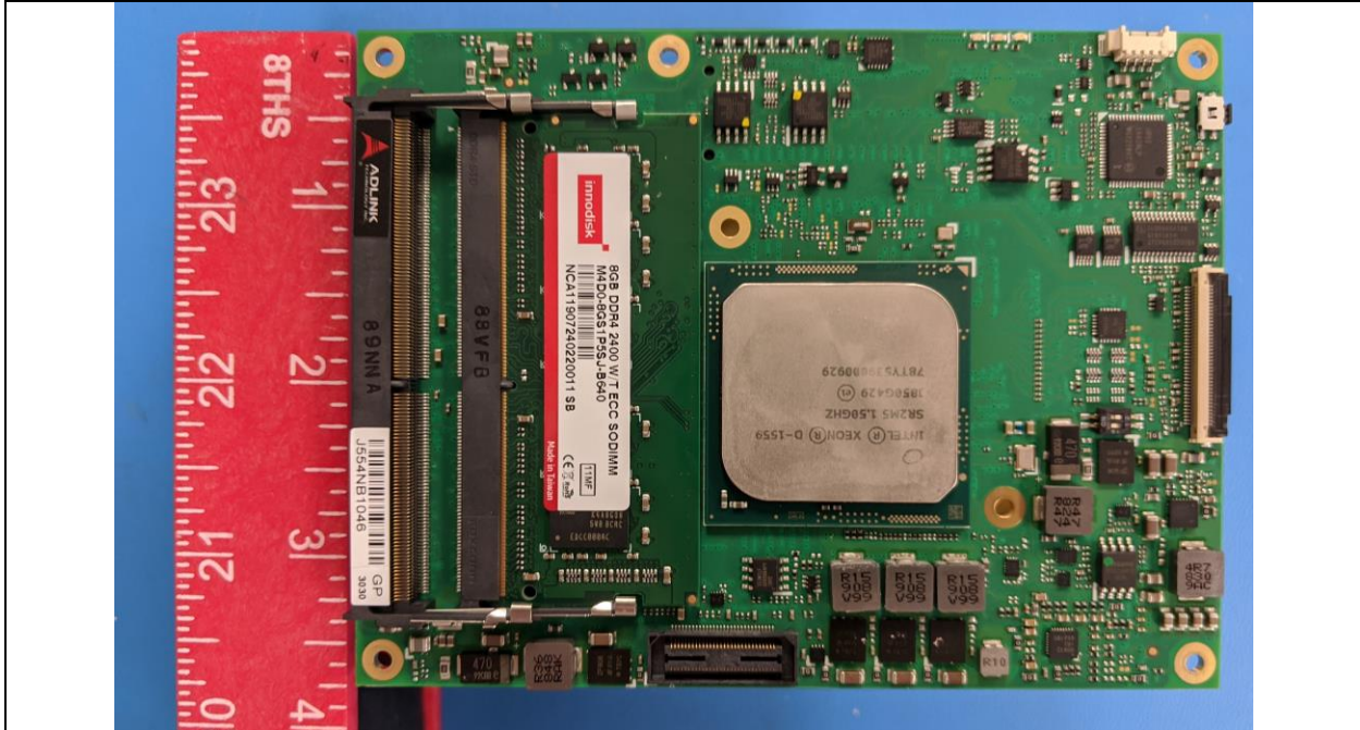
EUT ComE Front View
