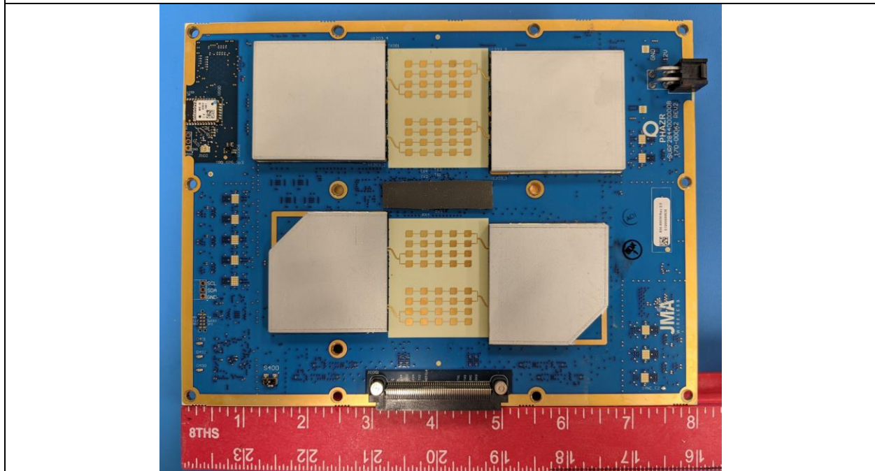
EUT IOTS Front View with shielding
