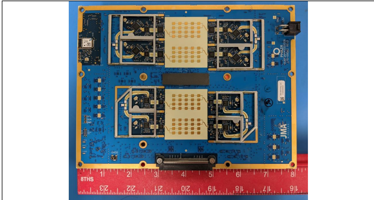
EUT IOTS Front View without shielding
