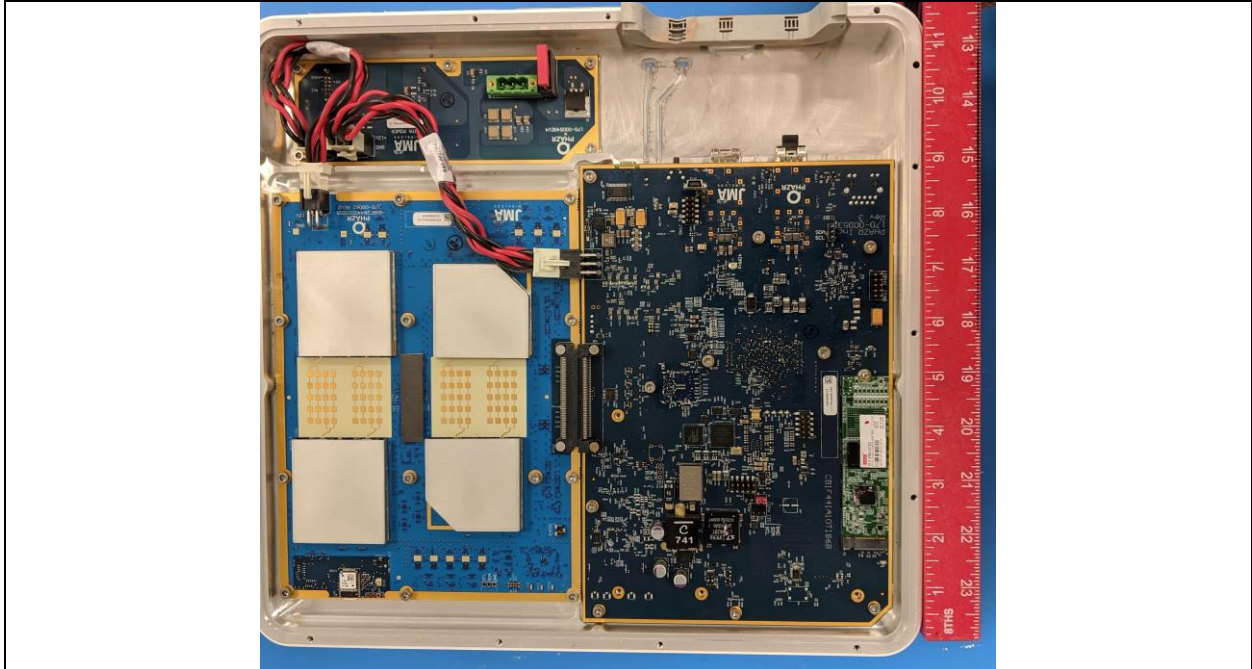
EUT Open case View
