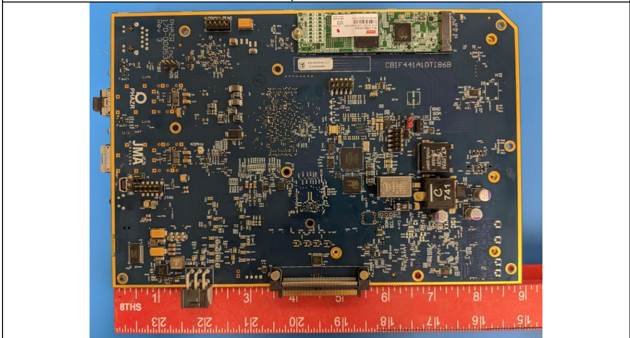
EUT IOTB Front View
