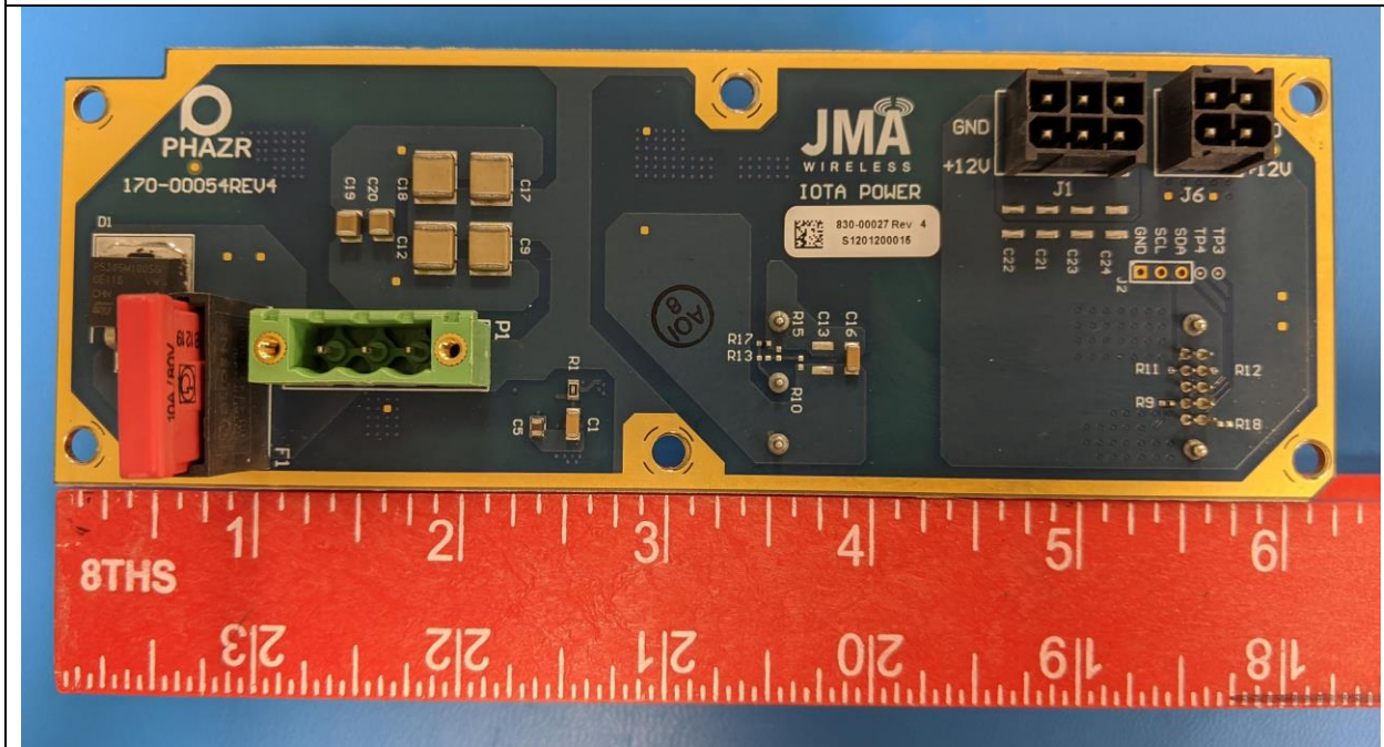
EUT IOTP Front View
