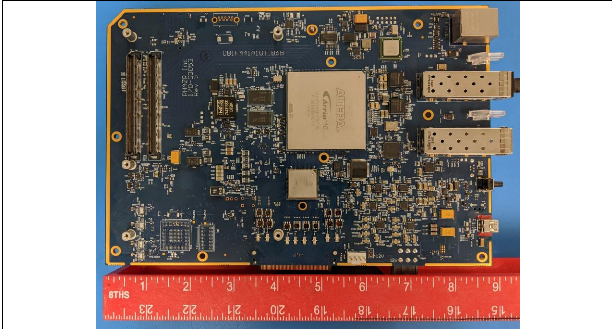
EUT IOTB Back View
