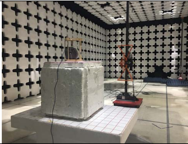
Radiated Emissions (>1GHz) - Rear View
