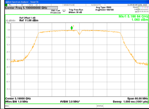
W52_11n40_Lower_Power Spectrum Density
