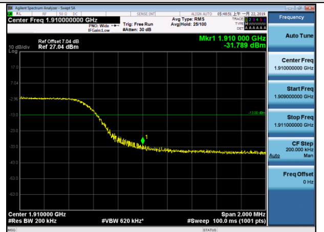
HCH_16QAM_50RB#0
