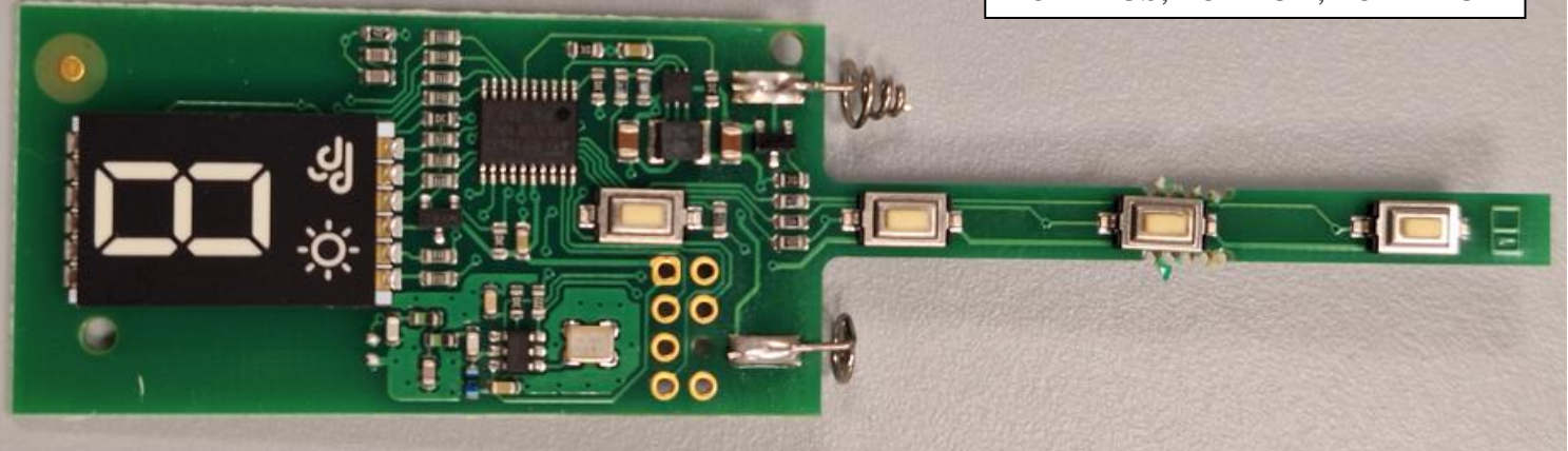
Board A4508_0R18 POP PLUS, POP LUX, POP P-LUX
