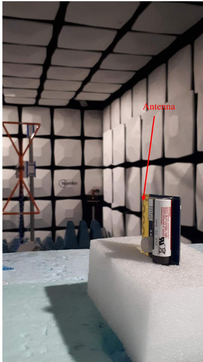
“Vertical” orientation – main orientation of antenna is vertical.
