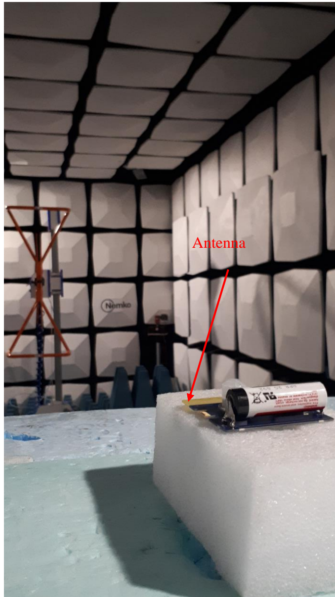
"Flat" orientation – main orientation of antenna is flat.
