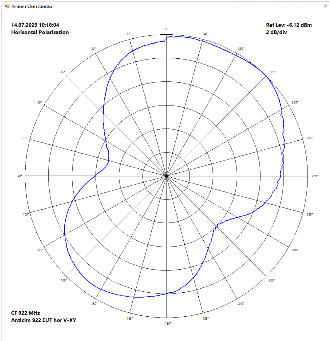
EUT "Horizontal" measurement antenna HP
