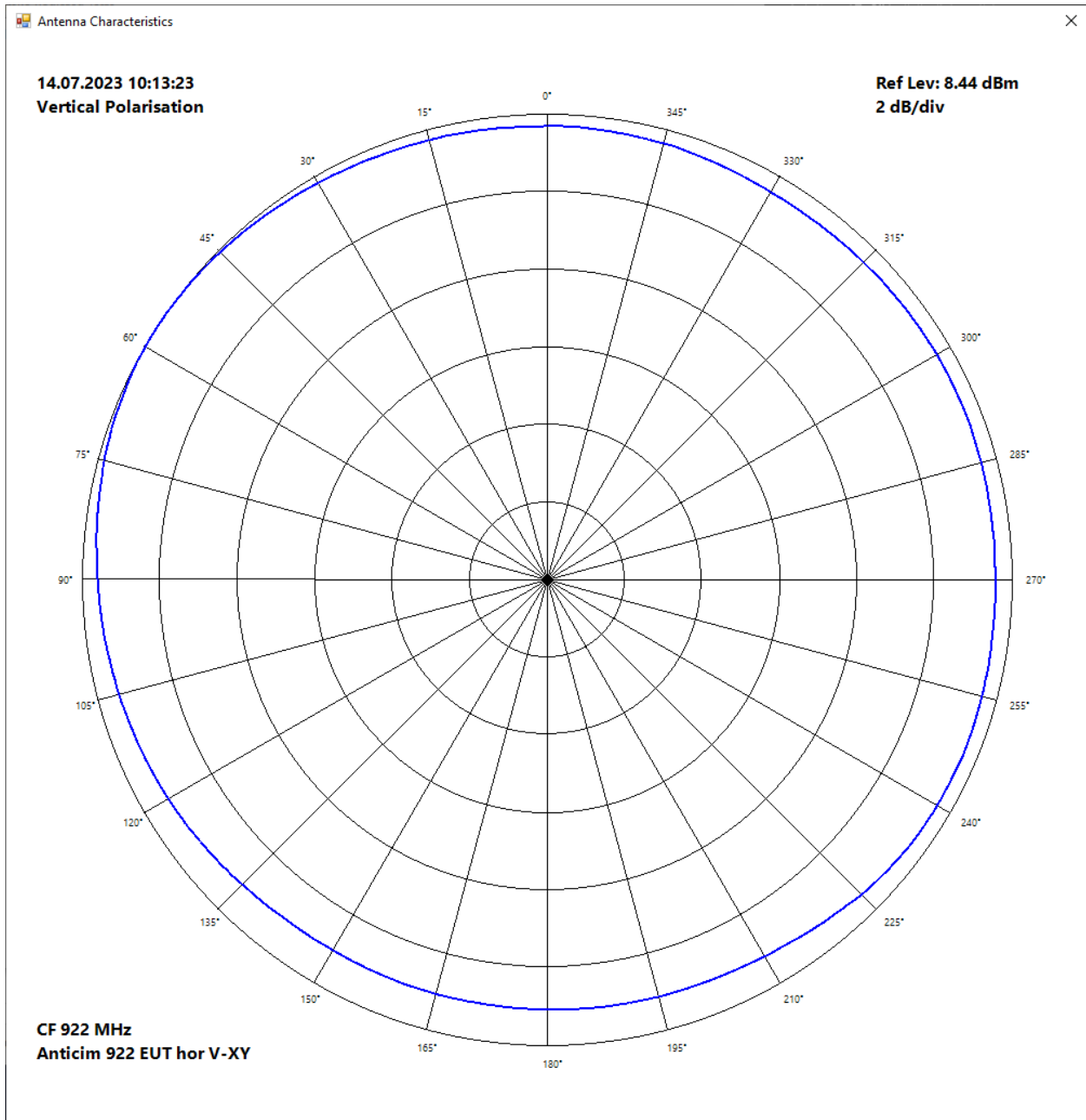
EUT "Horizontal" measurement antenna VP
