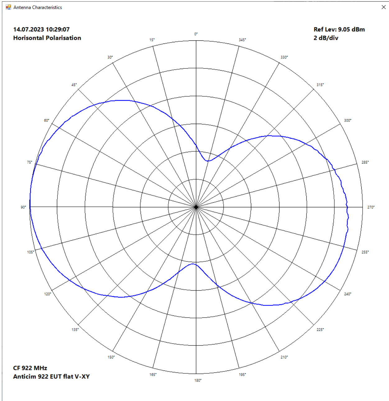
EUT "Flat" measurement antenna HP
