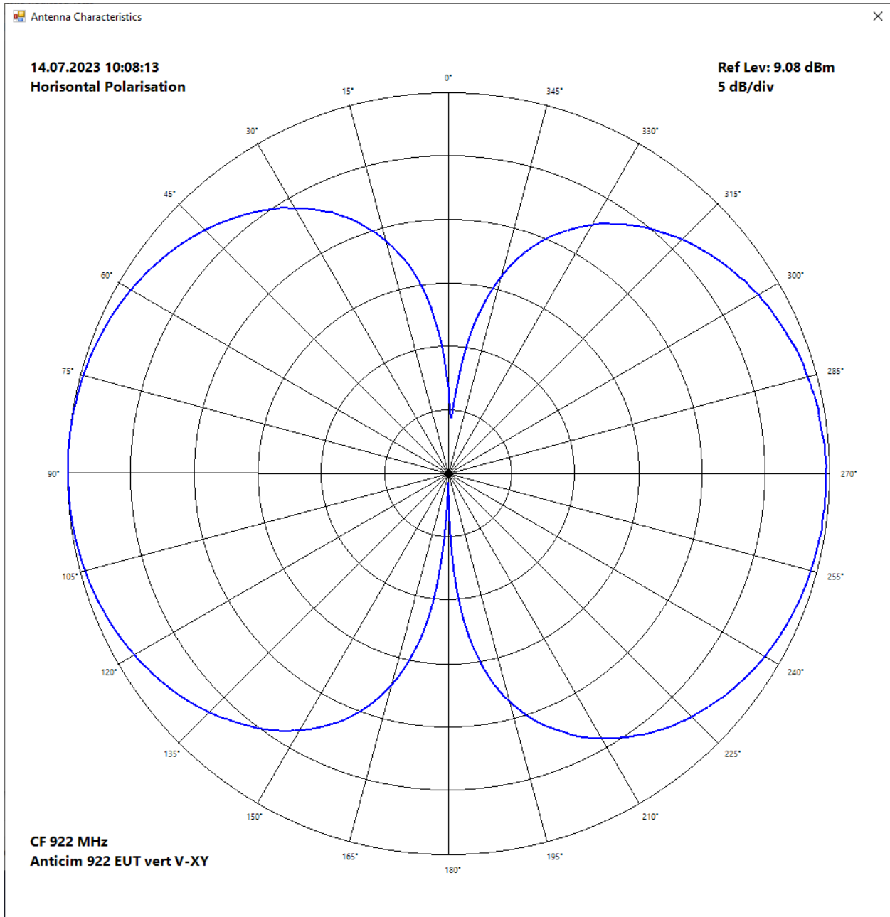
EUT "Vertical" measurement antenna HP
