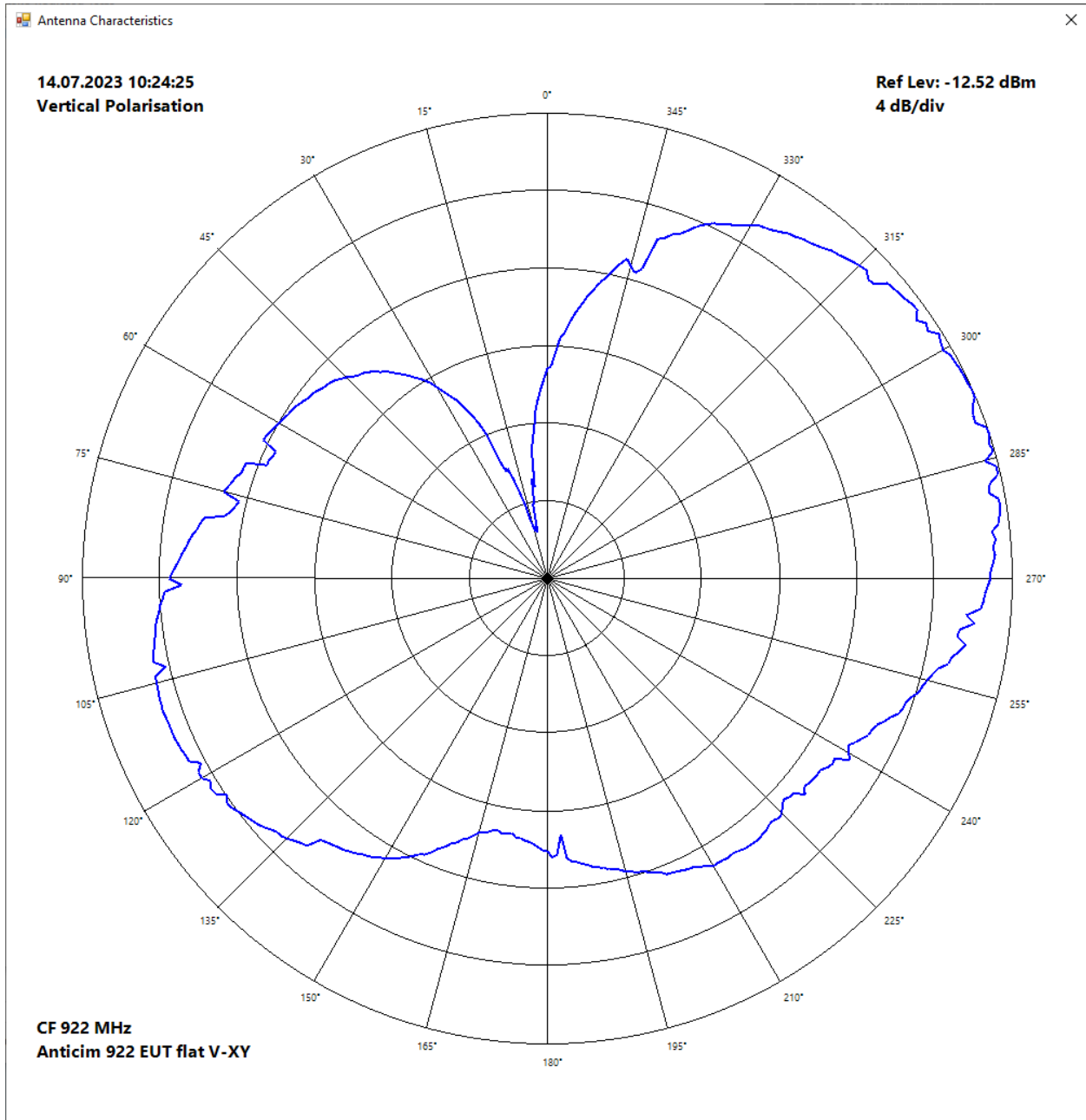
EUT "Flat" measurement antenna VP
