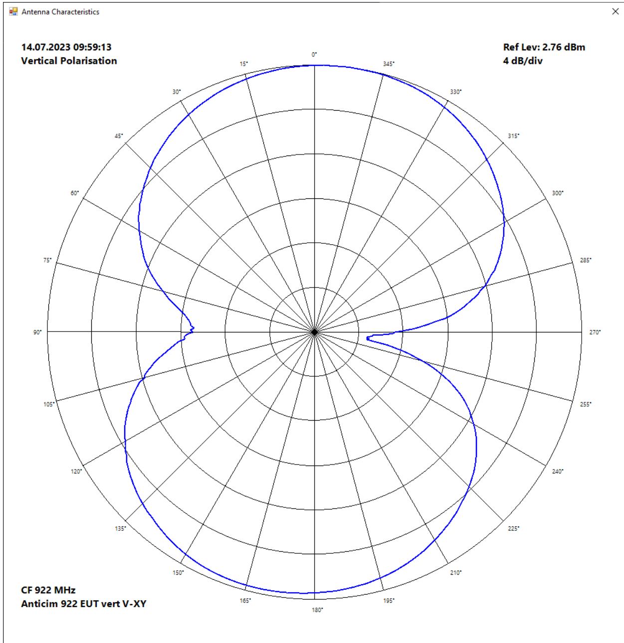
EUT "Vertical" measurement antenna VP
