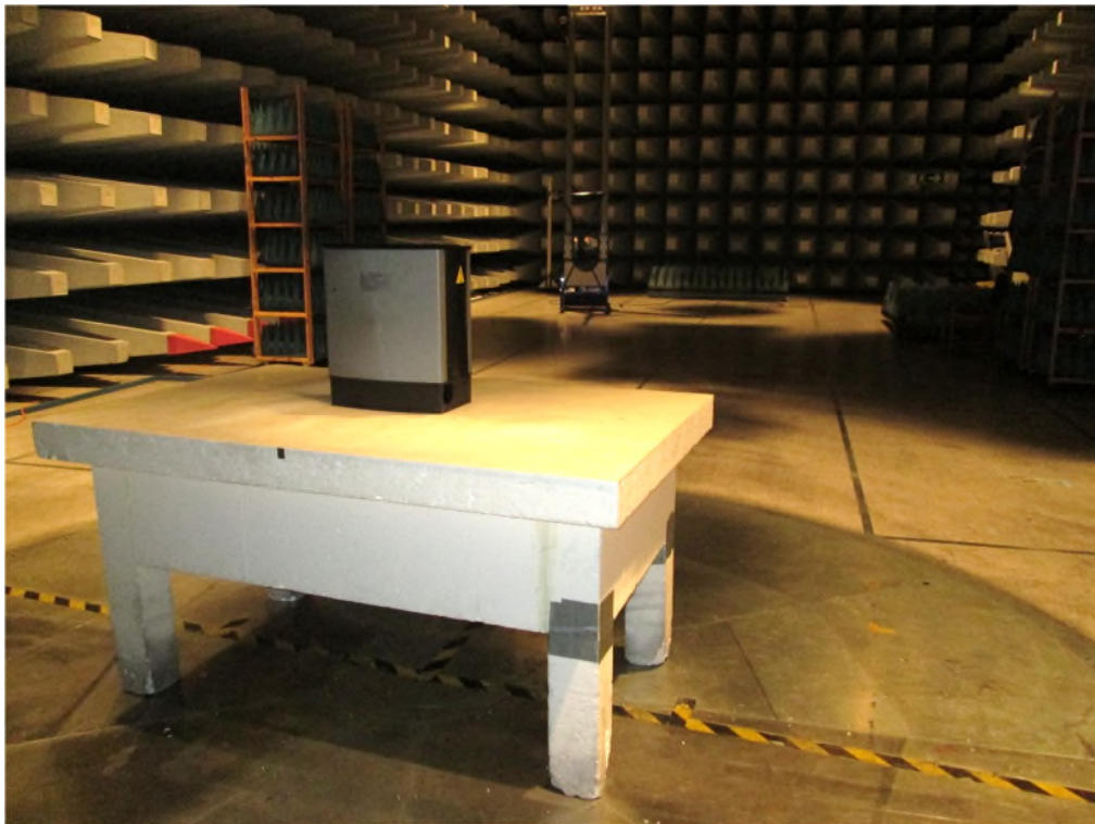
Photo 2.2 Test set up regarding measurement of radio frequency electromagnetic field below 1 GHz
