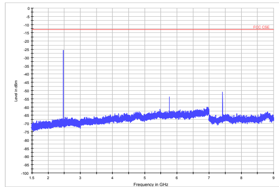
NB-IOT Band 5 CH-Low 1.5GHz-9GHz
