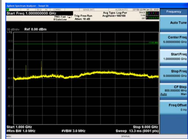
NB-IOT Band 5 CH-High 1 GHz-9GHz
