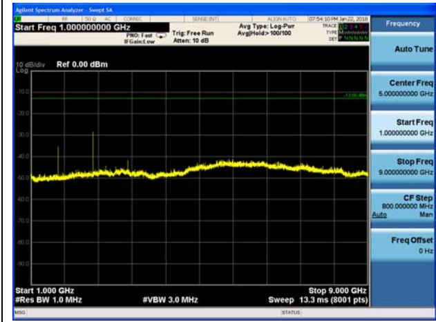
NB-IOT Band 5 CH-Middle 1GHz-9GHz
