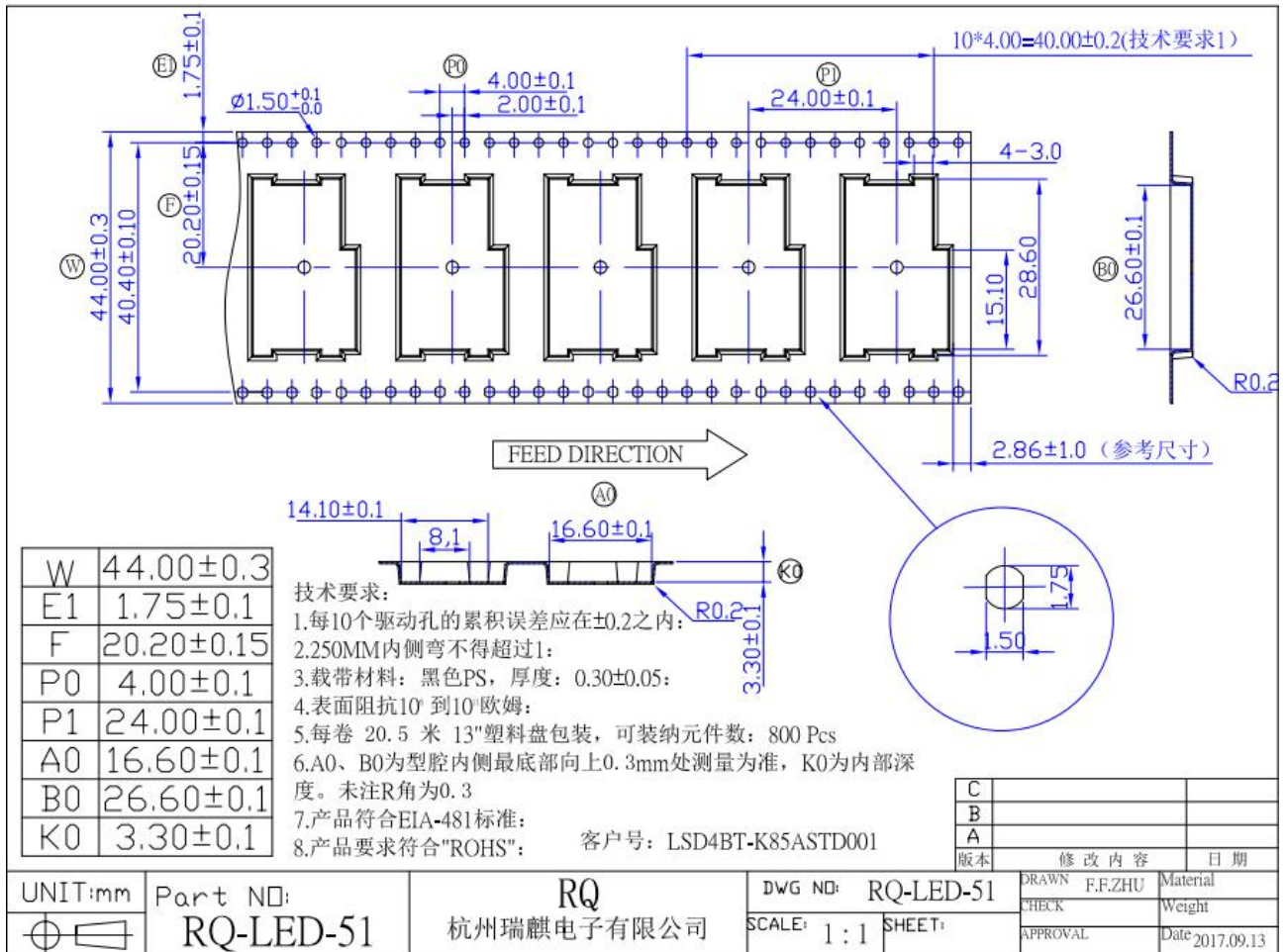
Fig. 6-1 Package Size
