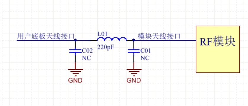
Figure 4 Module Antenna Interface Recommended Circuit
