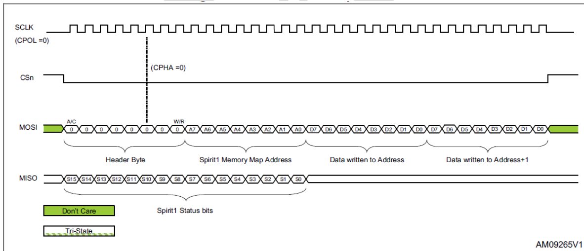
Figure 5 Module SPI Write Timing
