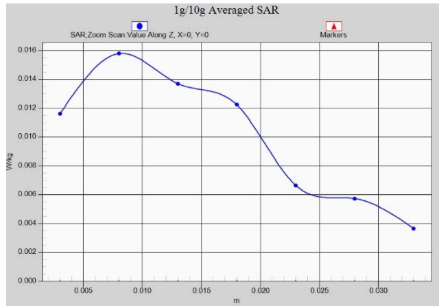
Fig.A.1- 13 Z-Scan at power reference point (Wifi2450)
