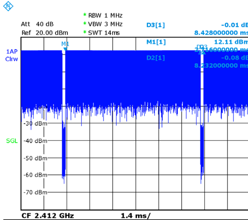
Picture 14.1 Duty factor plot (CH1 Head)
