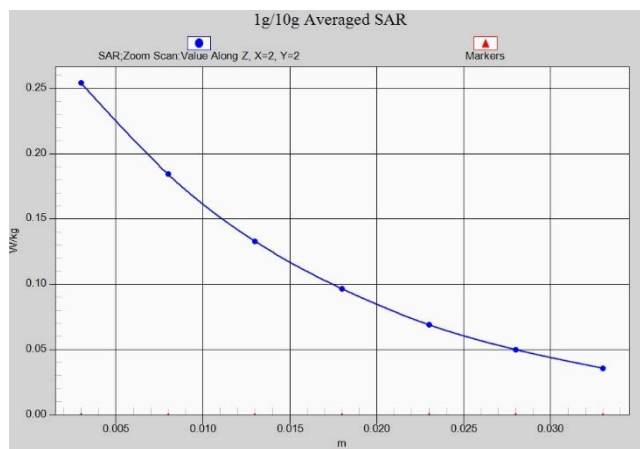
Fig.A.1- 14 Z-Scan at power reference point (Wifi2450)
