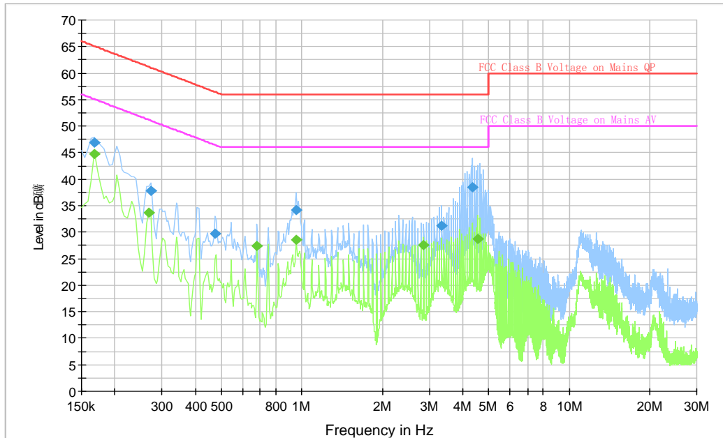
Fig A.6 Conducted Emission
