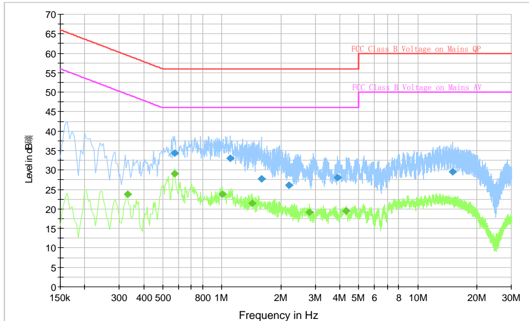
Fig A.5 Conducted Emission
