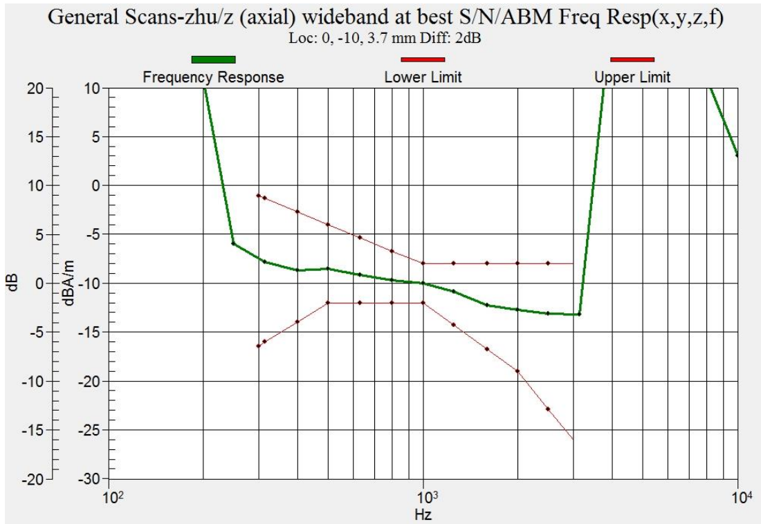
Figure C.11 Frequency Response of WiFi-2.4G
