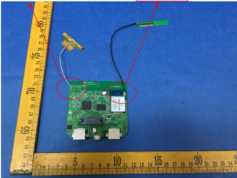
WIFI ANT.
