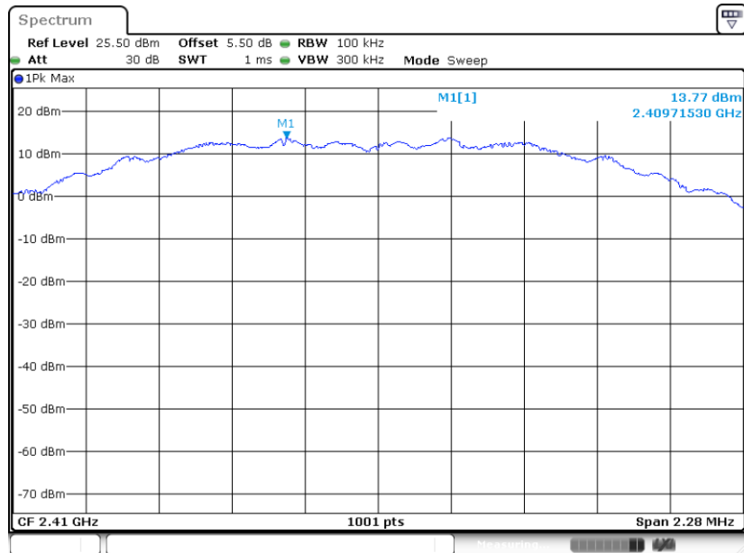
PSD 100kHz Plot on Channel 12
