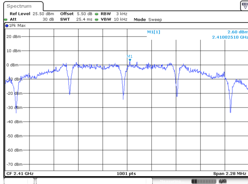
PSD 3kHz Plot on Channel 12
