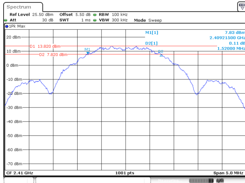
6 dB Bandwidth Plot on Channel 12
