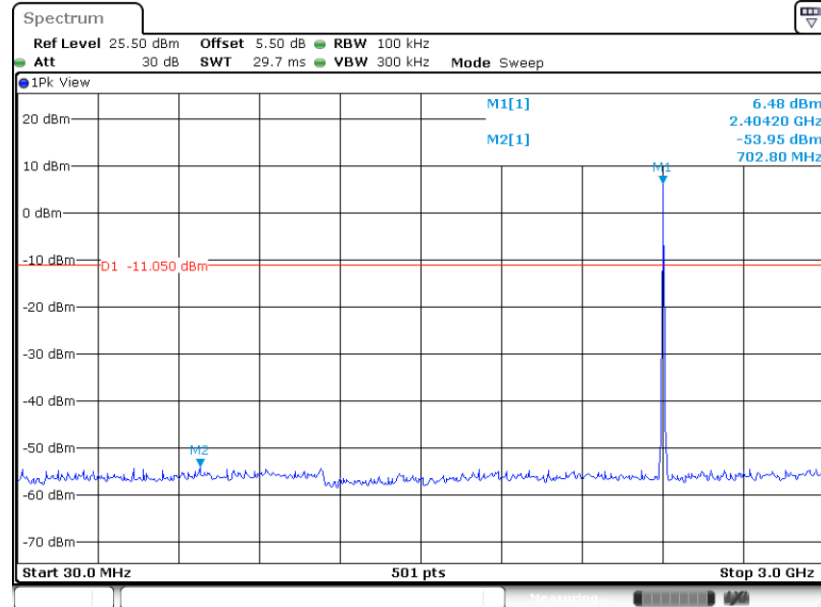
Conducted Spurious Emission Plot on Zigbee Channel 11
