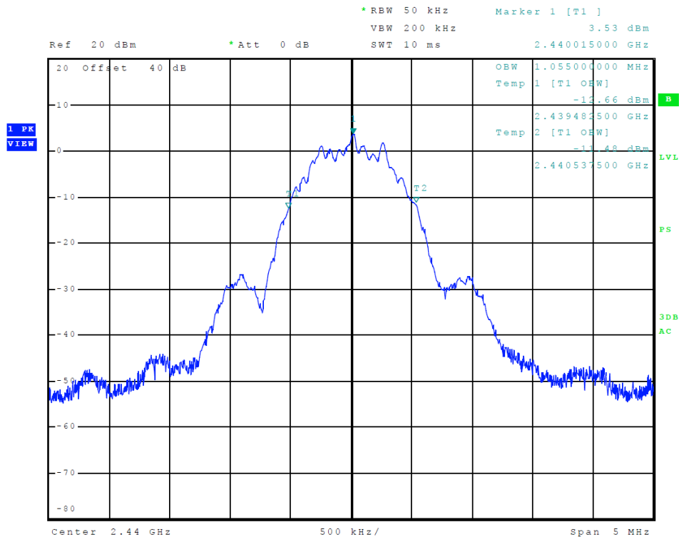
Figure 4 Plot of Transmitter 99% Occupied Bandwidth
