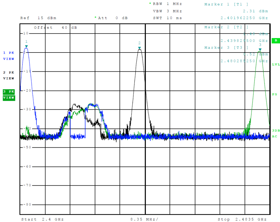
Figure 3 Plot of Operation across Frequency 2402-2480 MHz Band
