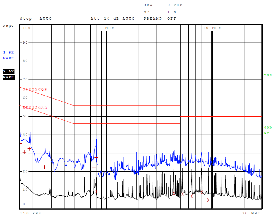
Figure 2 AC Line Conducted emissions of EUT line 2 (#2, EUT placed on WPT)
