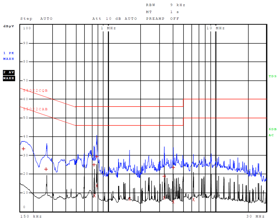
Figure 1 AC Line Conducted emissions of EUT line 1 (#2, EUT placed on WPT)
