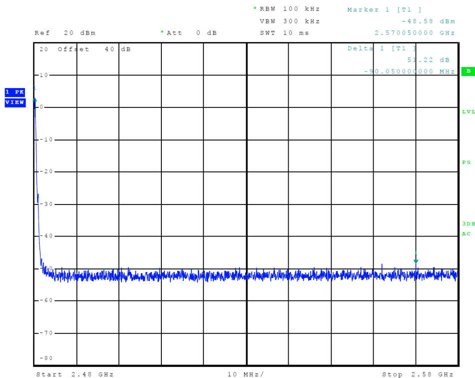
Figure 6 Plot of Transmitter High Band Edge Compliance
