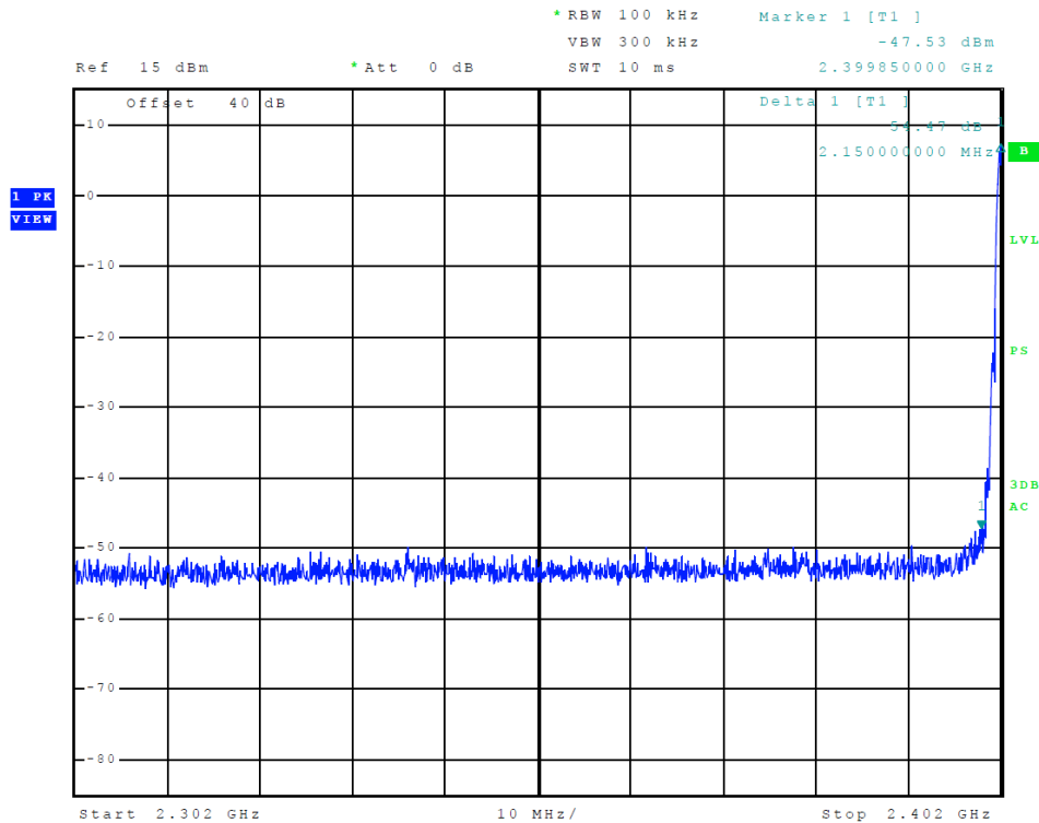
Figure 5 Plot of Transmitter Low Band Edge Compliance
