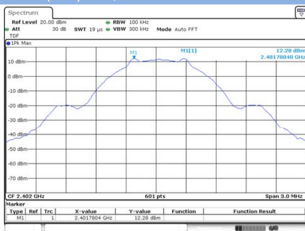
GFSK (BLE) CH0, Carrier level
