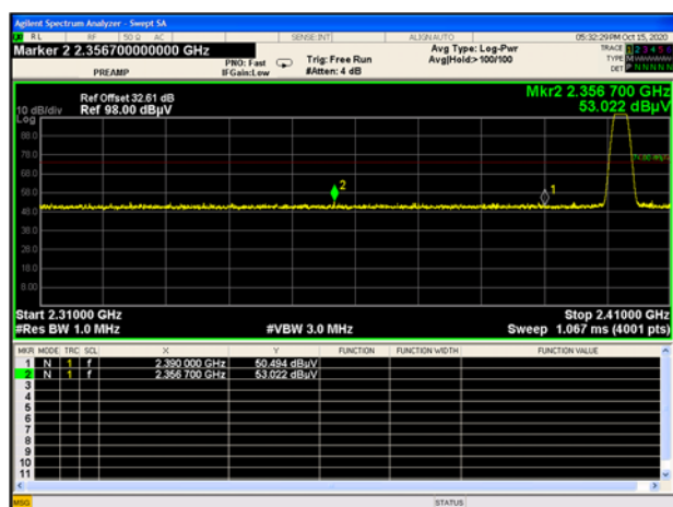
GFSK (BLE) CH0, PEAK
