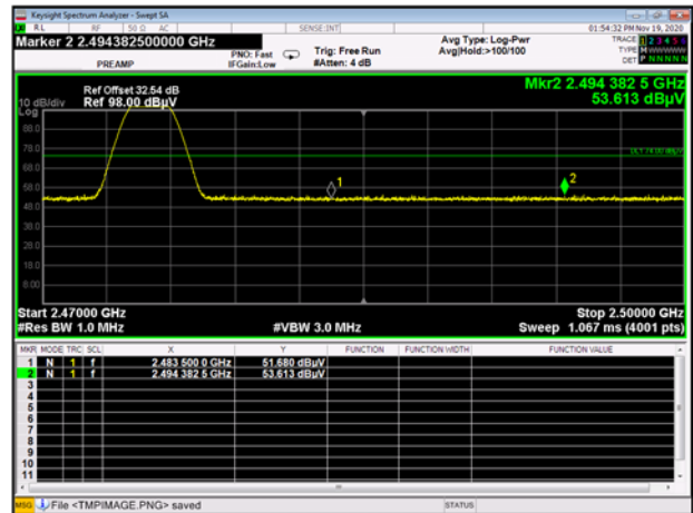
O-QPSK (Zigbee) CH25, PEAK
