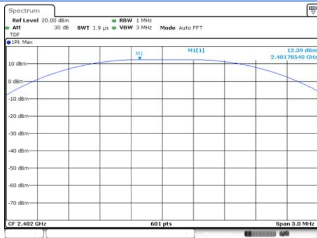
GFSK (BLE) CH0
