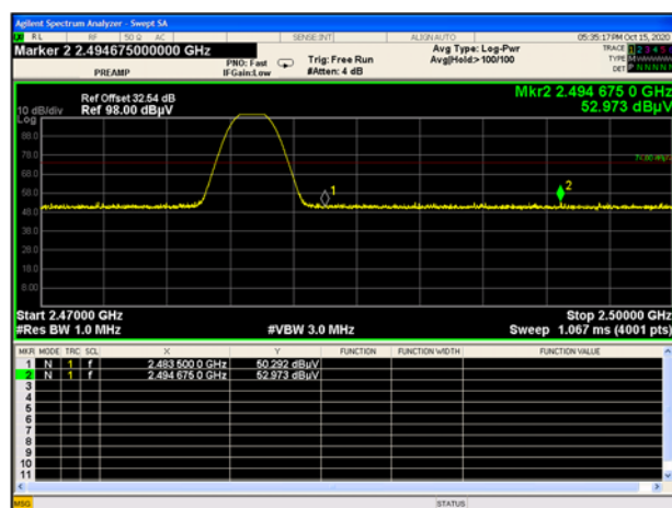
GFSK (BLE) CH39, PEAK
