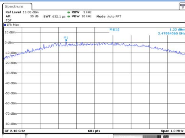
GFSK (BLE) CH39
