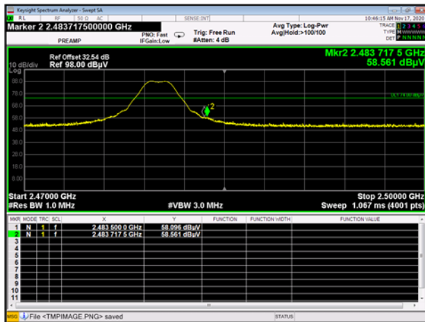
O-QPSK (Zigbee) CH26, PEAK
