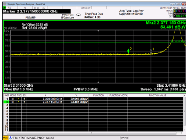
O-QPSK (Zigbee) CH11, PEAK
