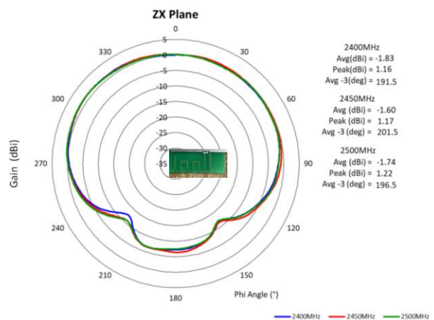
Radiation pattern Z-X plane
