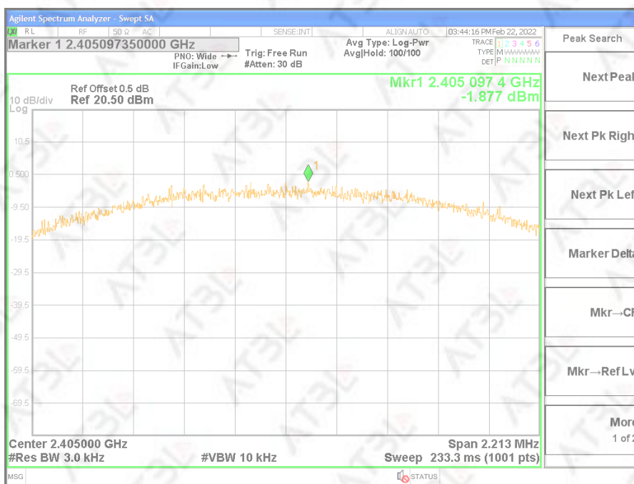
Mode1 CH11
