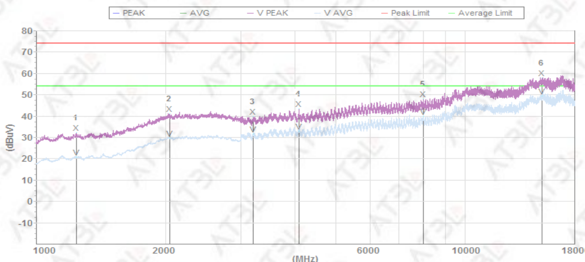
Mode 1 Vertical
