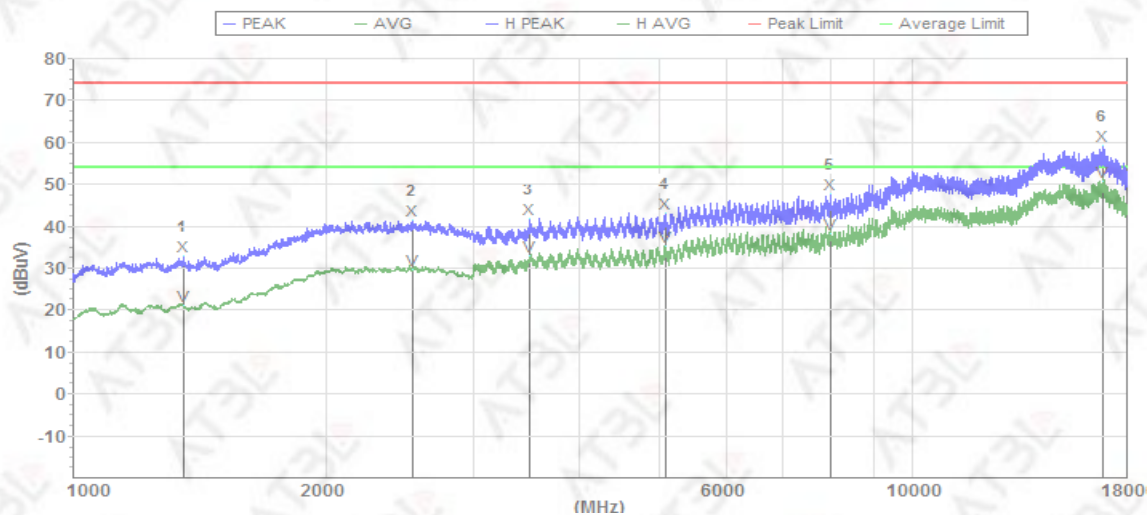
Mode 3 Horizontal
