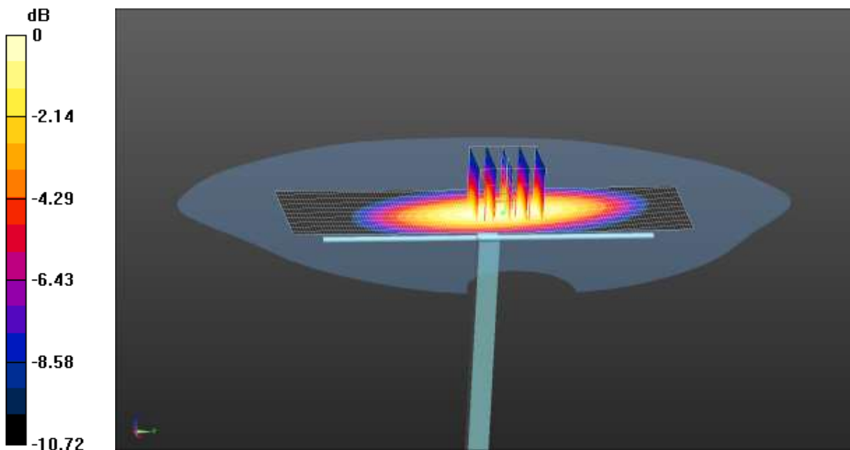
0 dB = 0.941 W/kg = -0.26 dBW/kg
