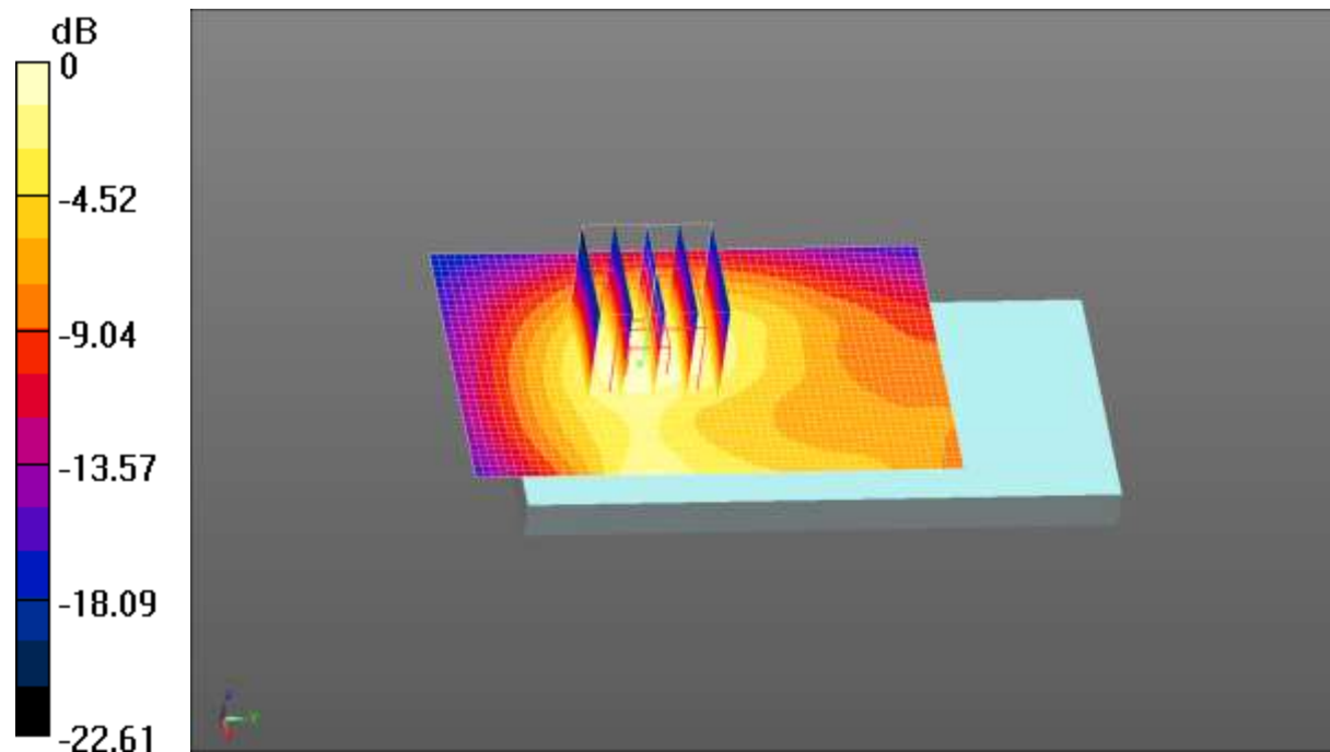
0 dB = 0.191 W/kg = -7.19 dBW/kg
