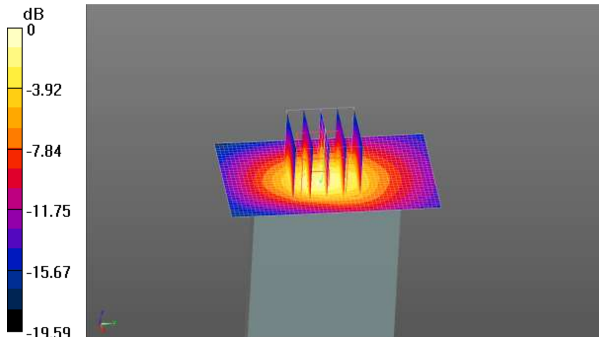
0 dB = 1.82 W/kg = 2.60 dBW/kg
