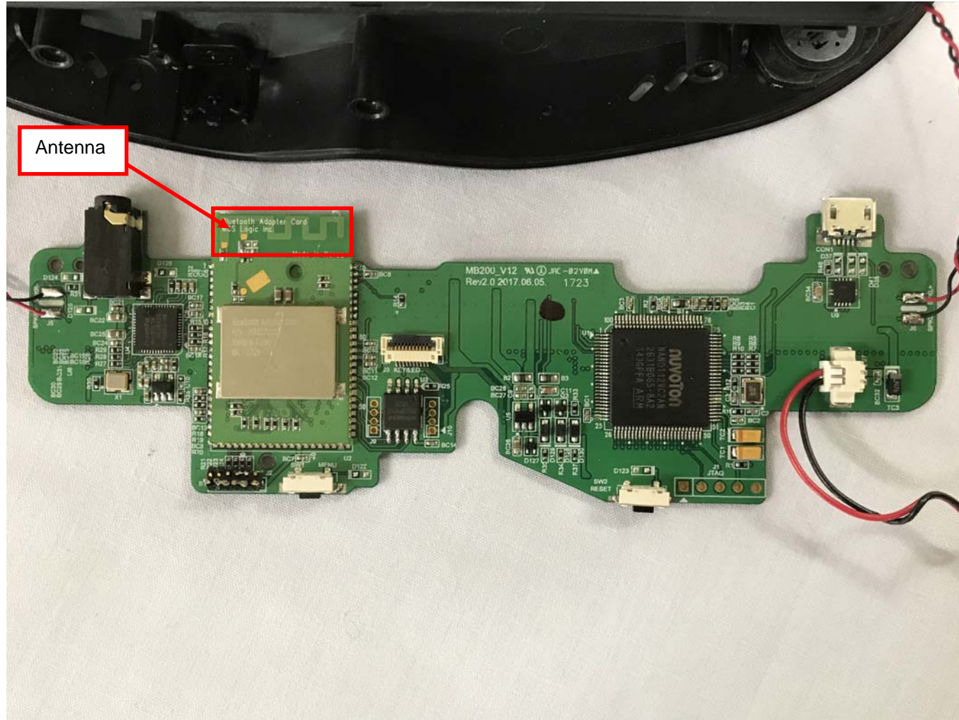
[Antenna portion]
