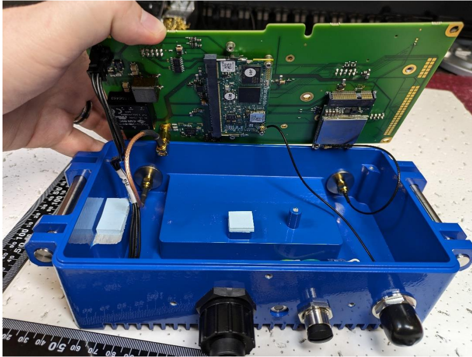
Figure 3 - Industrial Edge Machine - Internal RF Connection
