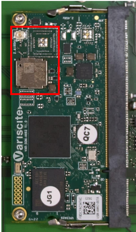
Figure 6 - Industrial Edge Machine - Wi-Fi and Bluetooth Radio Module
