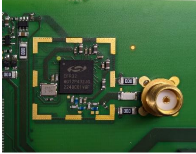
Figure 5 - Industrial Edge Machine – 802.15.4 and BLE Radio Circuit
