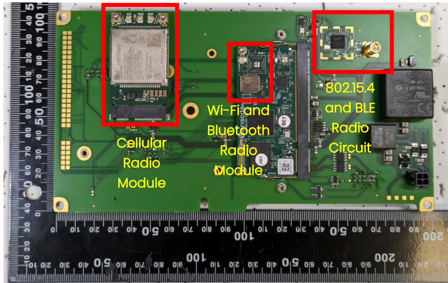
Figure 2 - Industrial Edge Machine - Main PCB - Bottom
