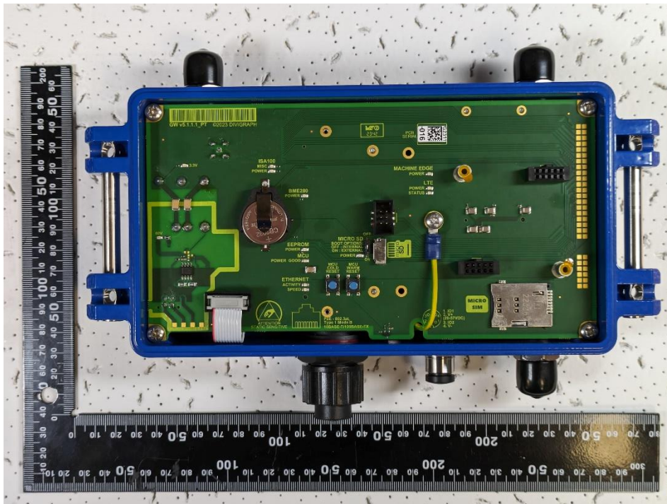
Figure 4 - Industrial Edge Machine - Internal Assembly
