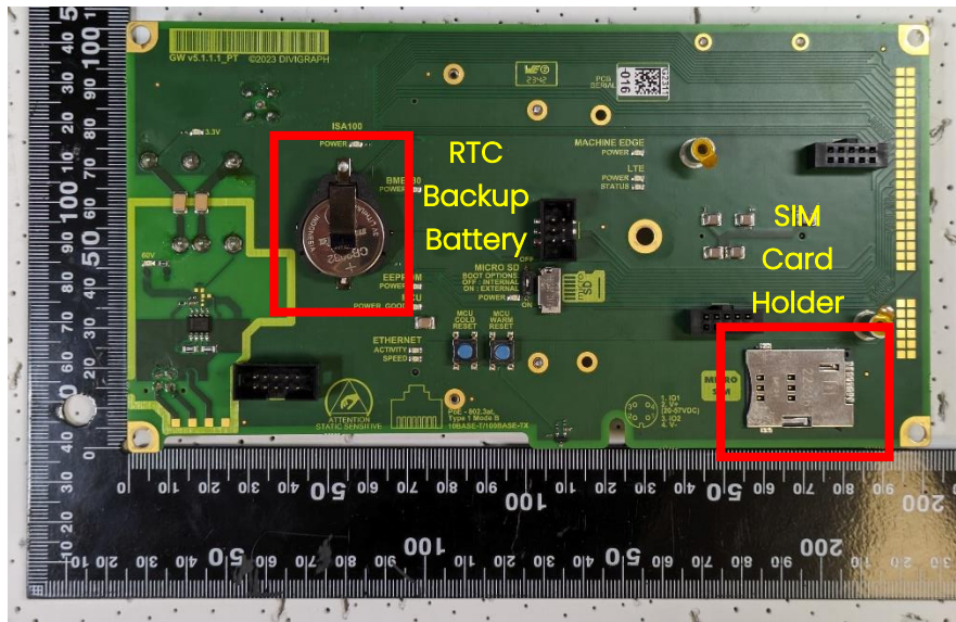
Figure 1 - Industrial Edge Machine - Main PCB - Top
