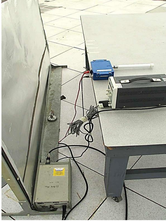
24VDC Test Setup; Side View
