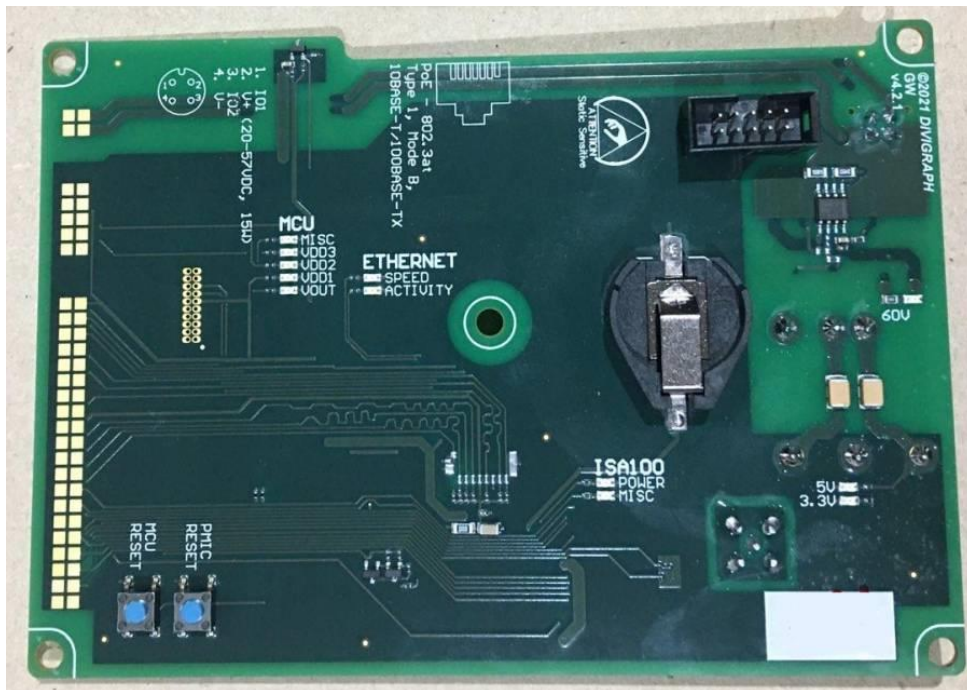
Figure 2 - PCB Bottom
