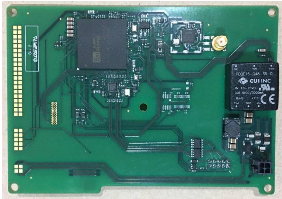
Figure 1 - PCB Top
