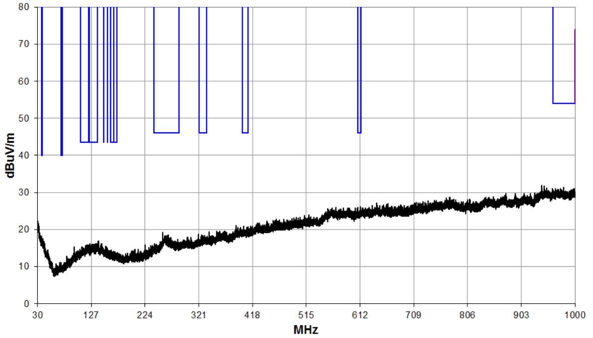
30 MHz – 1 GHz
