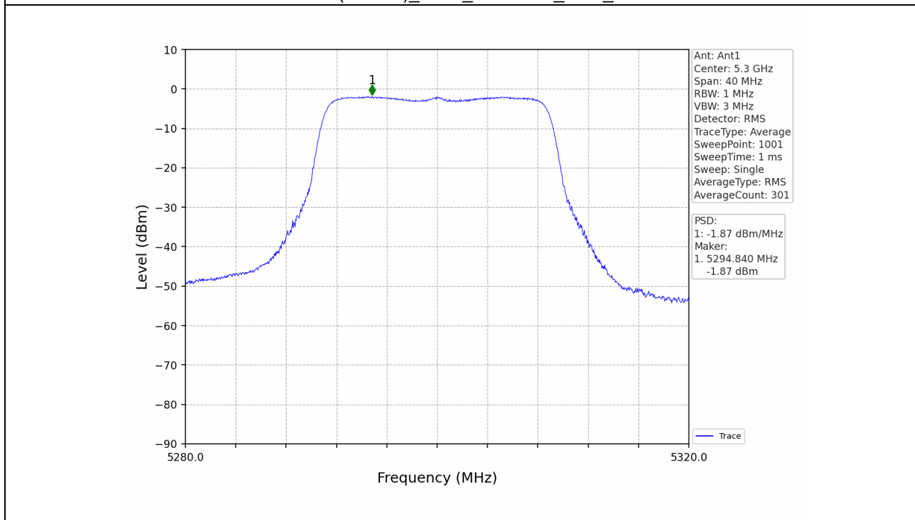
802.11ac(VHT20)_MCH_5300MHz_Ant1_NTNV
