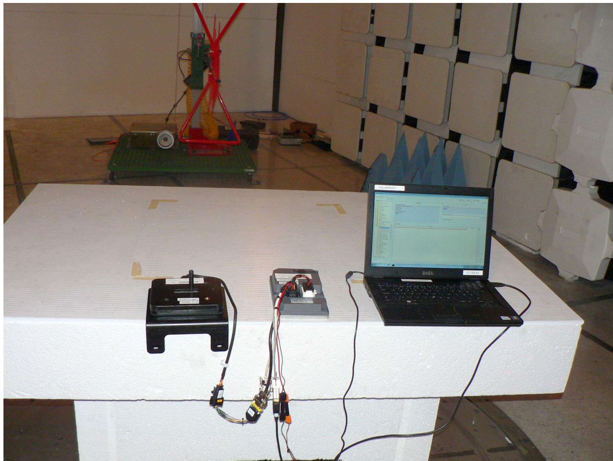
VMC30 TX Spurious 30-1000
