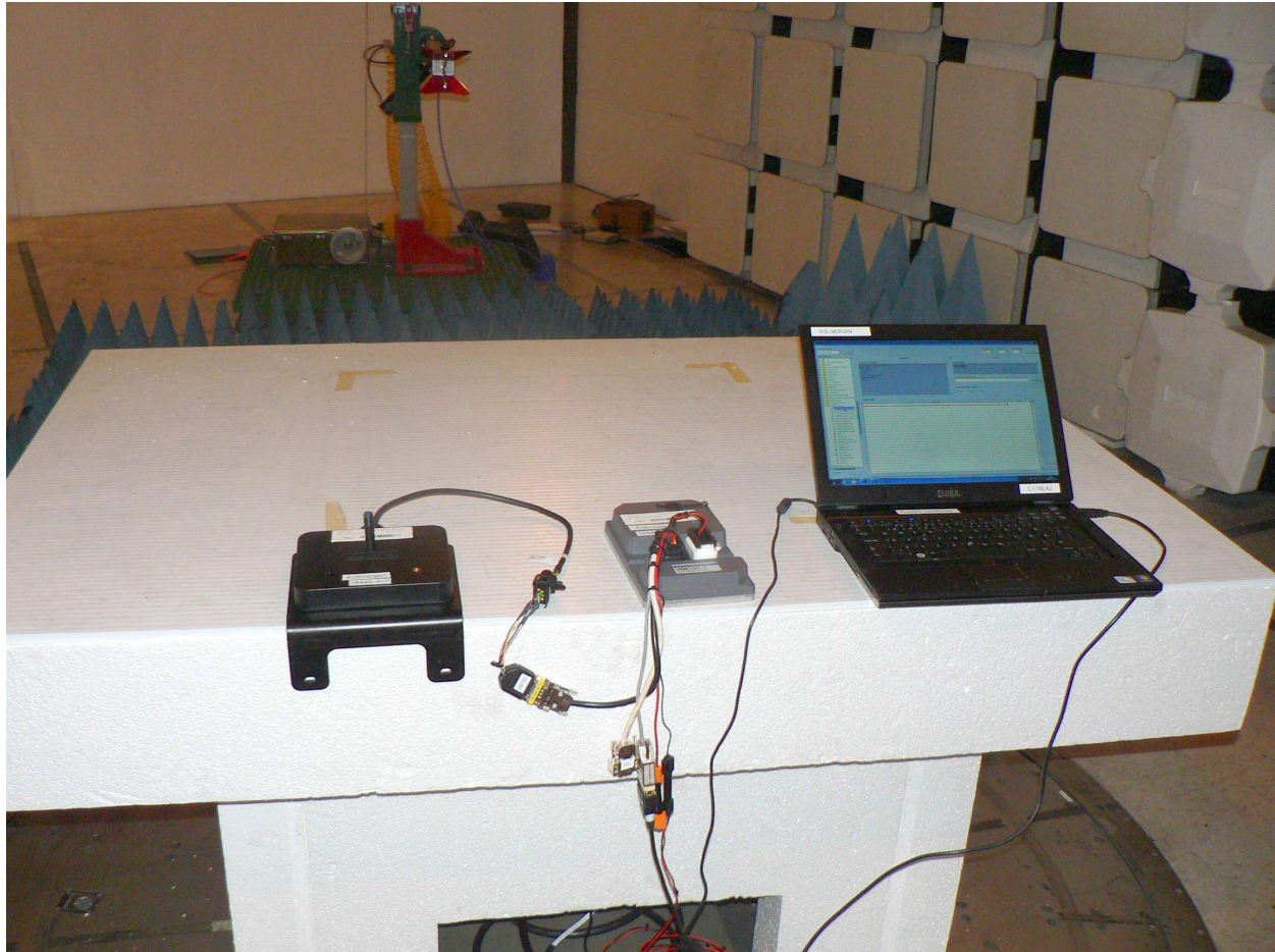
VMC300 TX Spurious 1-18G Back
