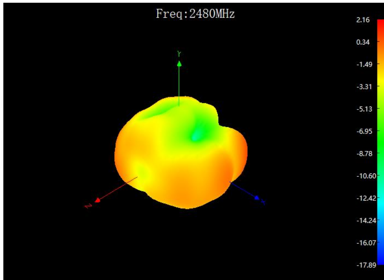
3D-Etotal (2480Mhz)
