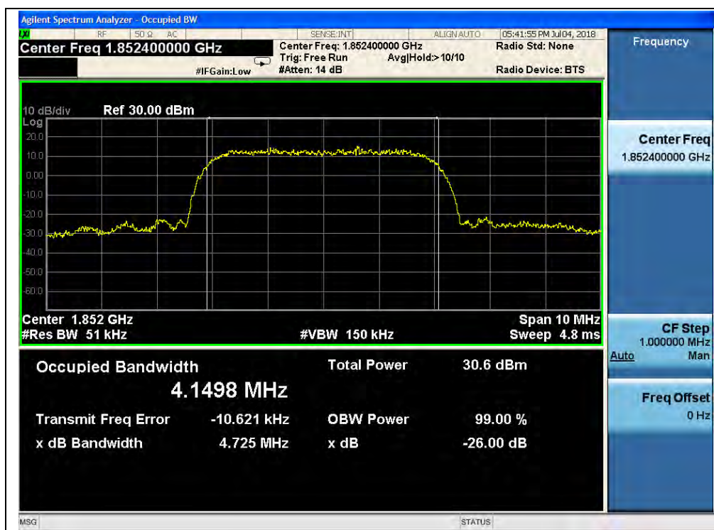
(Plot R1, HSPA+ 1900MHz, Channel = 9262)
