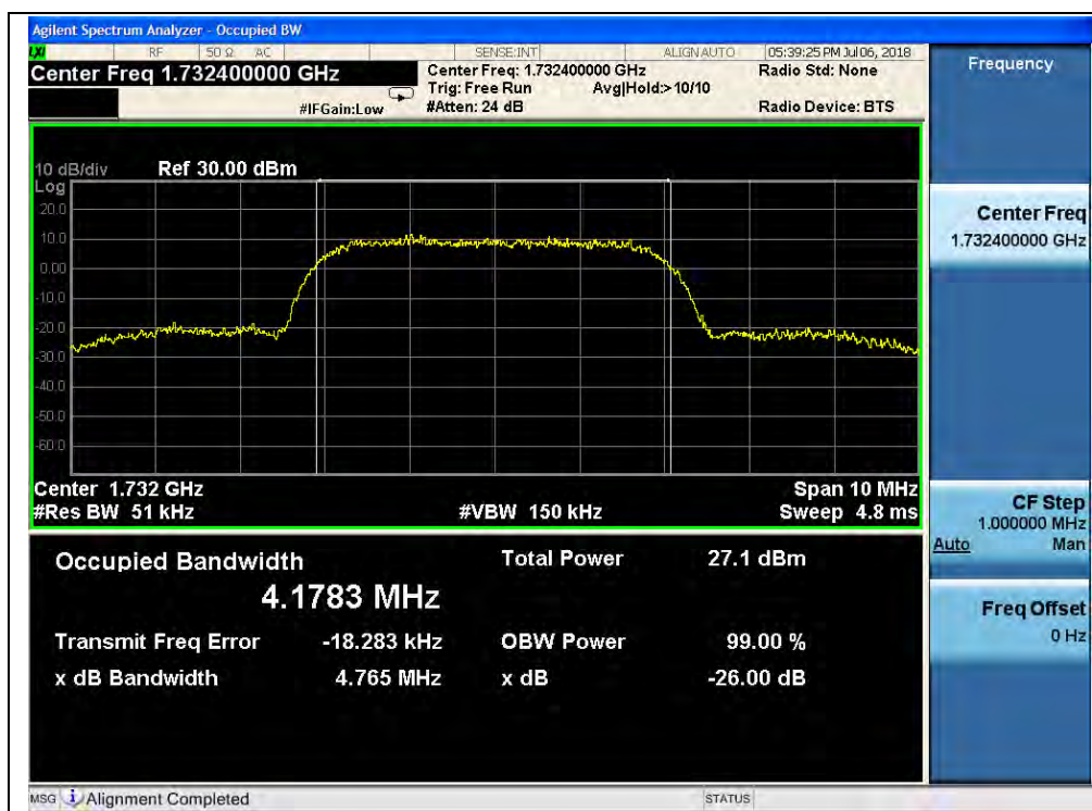
(Plot Q2, HSPA+ 1700 MHz, Channel = 1412)
