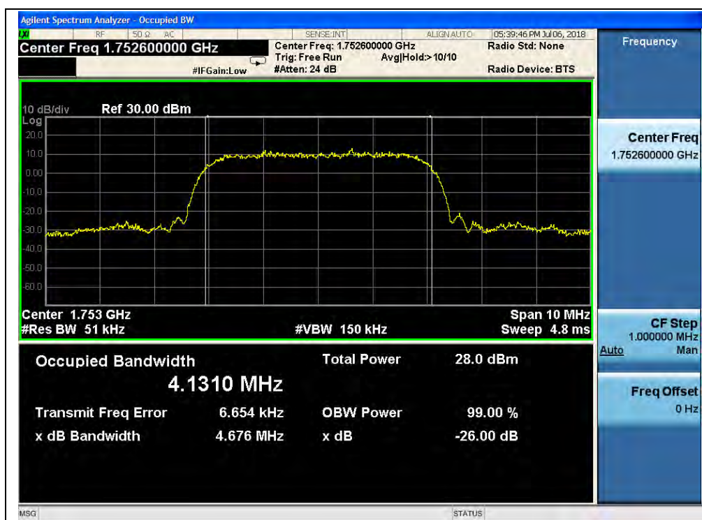
(Plot Q3, HSPA+ 1700MHz, Channel = 1513)
