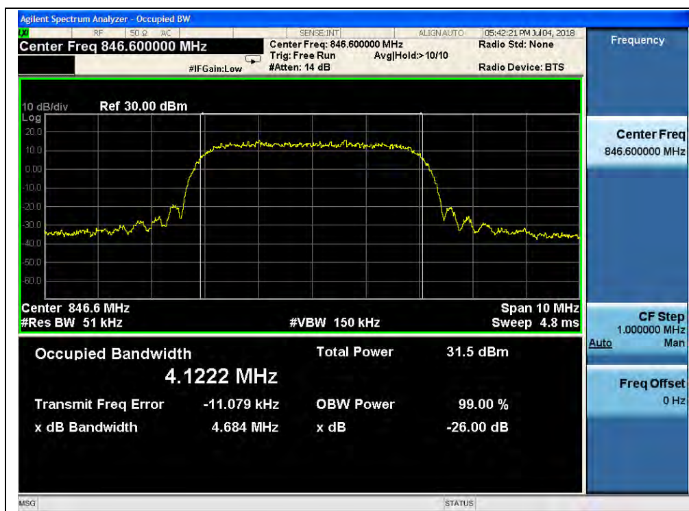
(Plot P3, HSPA+ 850MHz, Channel = 4233)
