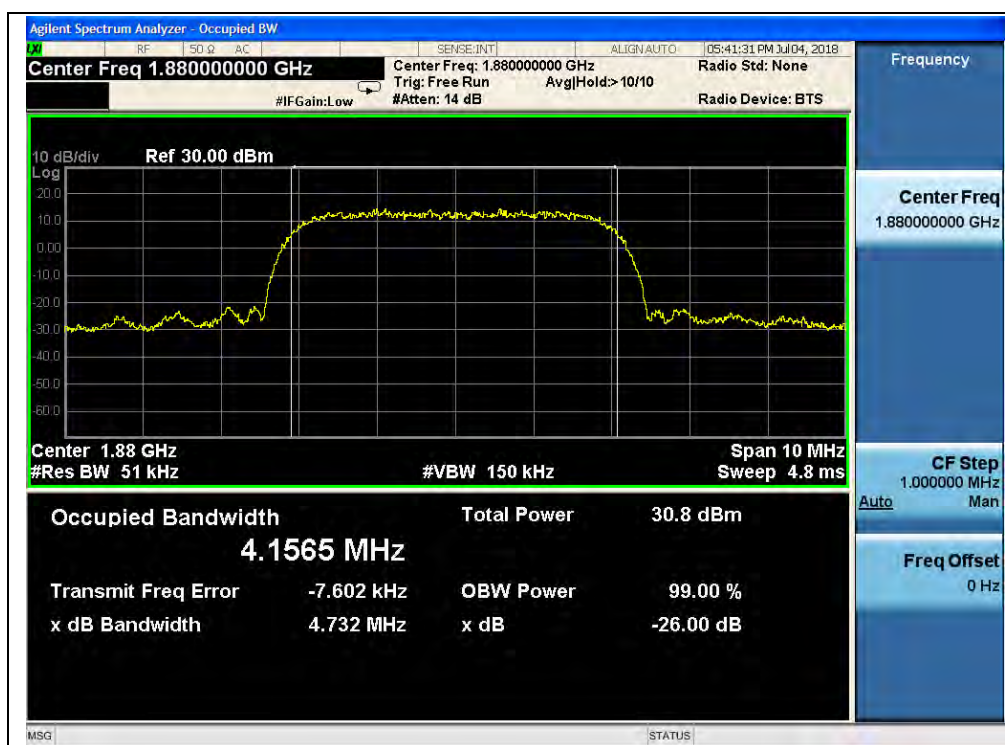
(Plot R2, HSPA+ 1900 MHz, Channel = 9400)
