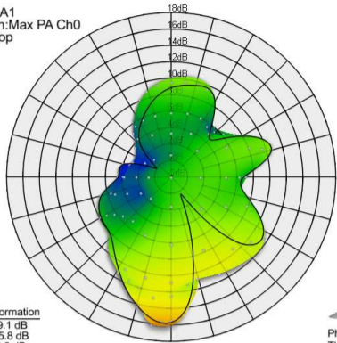
Channel 0, Bottom Antenna from the front
