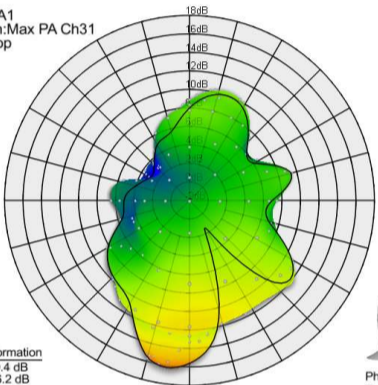
Channel 31, Bottom Antenna from the front
