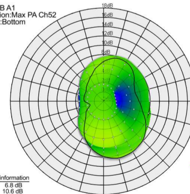
Channel 52, Bottom Antenna from the top
