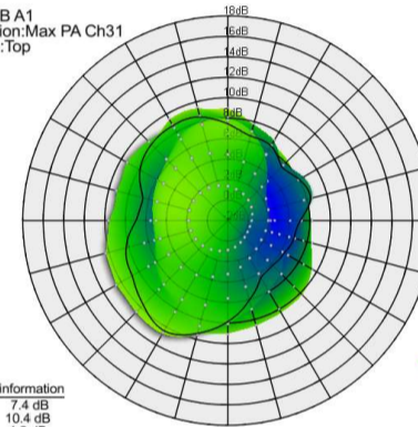
Channel 31, Bottom Antenna from the top
