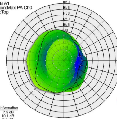
Channel 0, Bottom Antenna from the top
