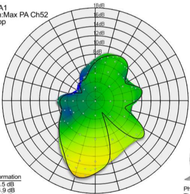
Channel 52, Bottom Antenna from the front
