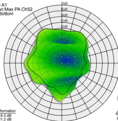
Channel 52, Bottom Antenna from the side
