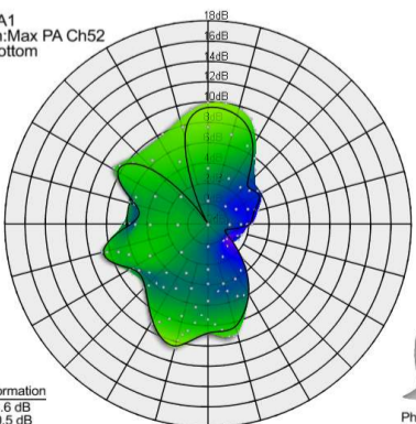
Channel 52, Bottom Antenna from the front
