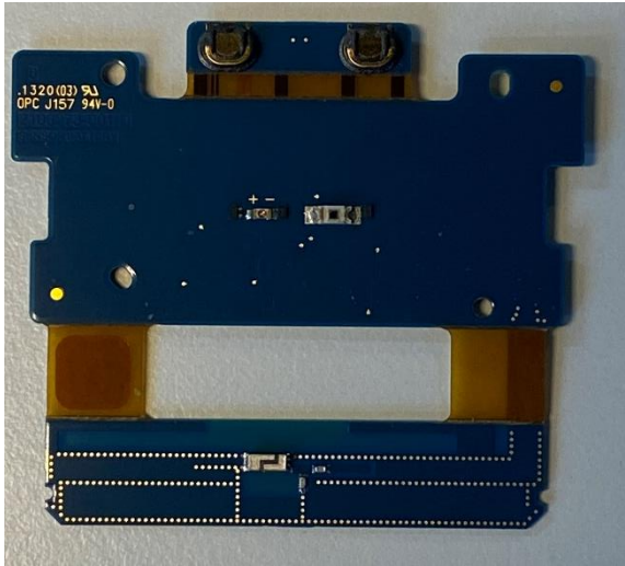
PWB bottom side
