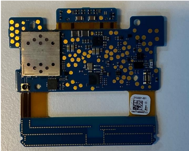
PWB (printed wiring board) top side with RF shield
