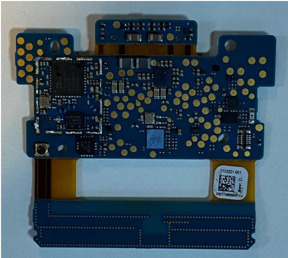
PWB top side without RF shield
