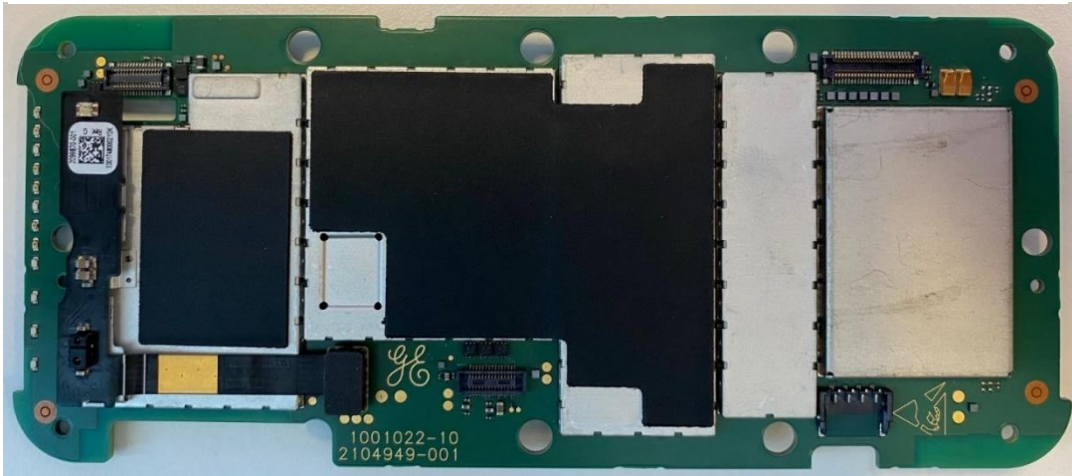
PWB top with RF shields
