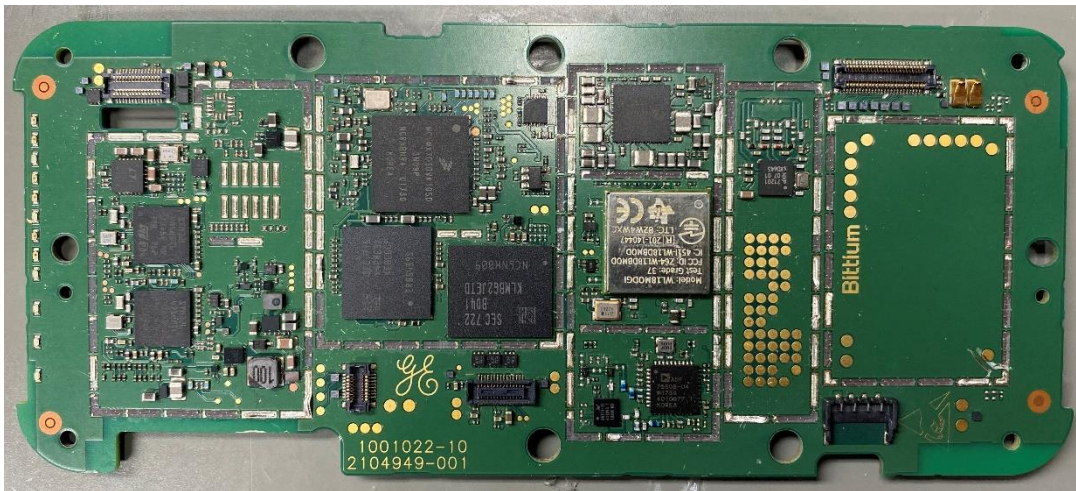
PWB top RF shields removed
