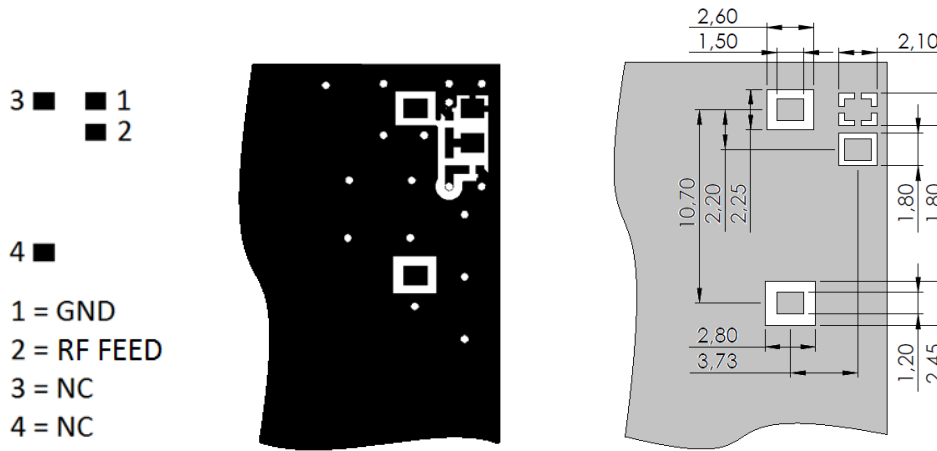
Pin configuration
