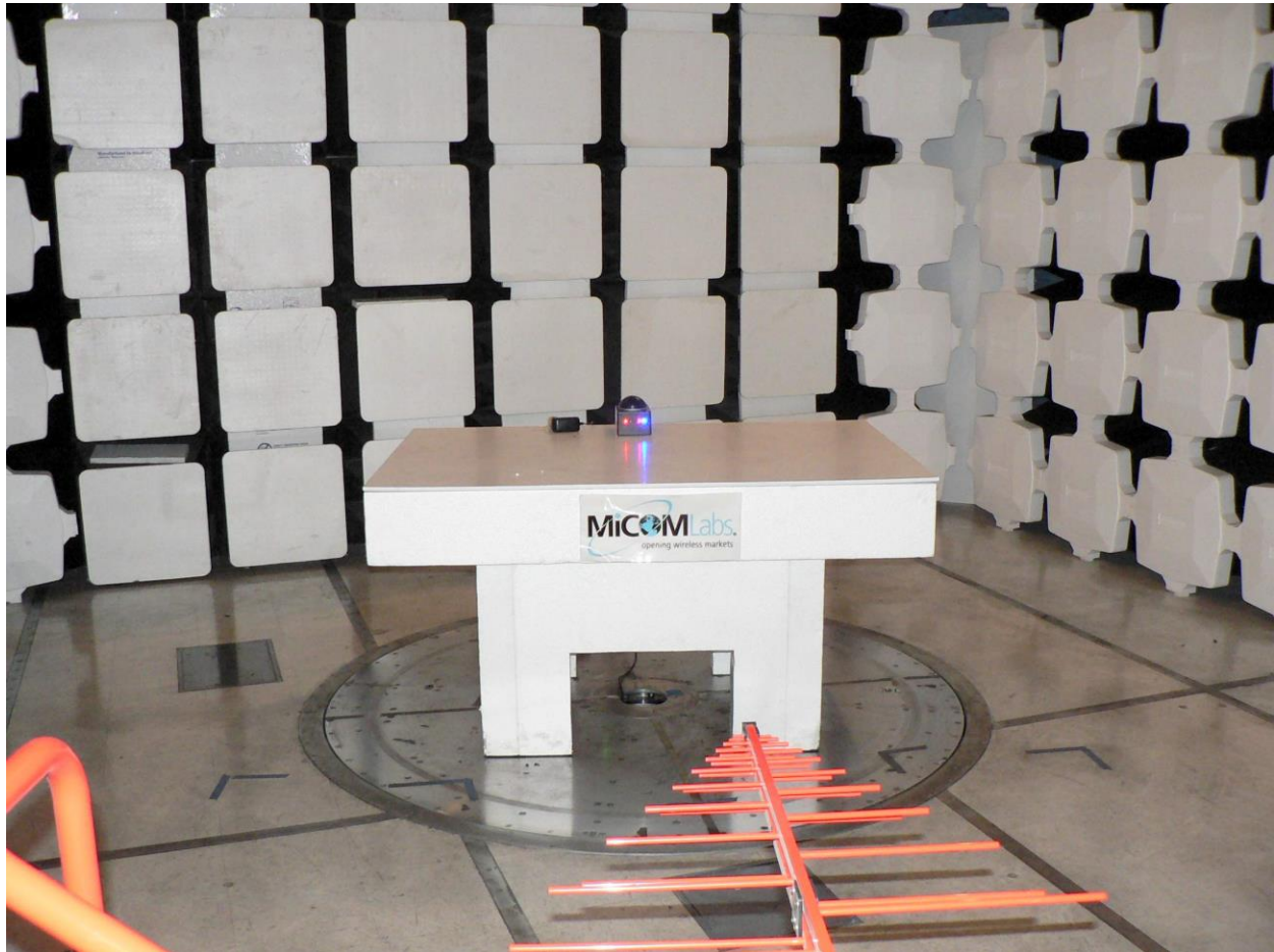
DVD41POE Digital Emissions 30-1000 MHz
